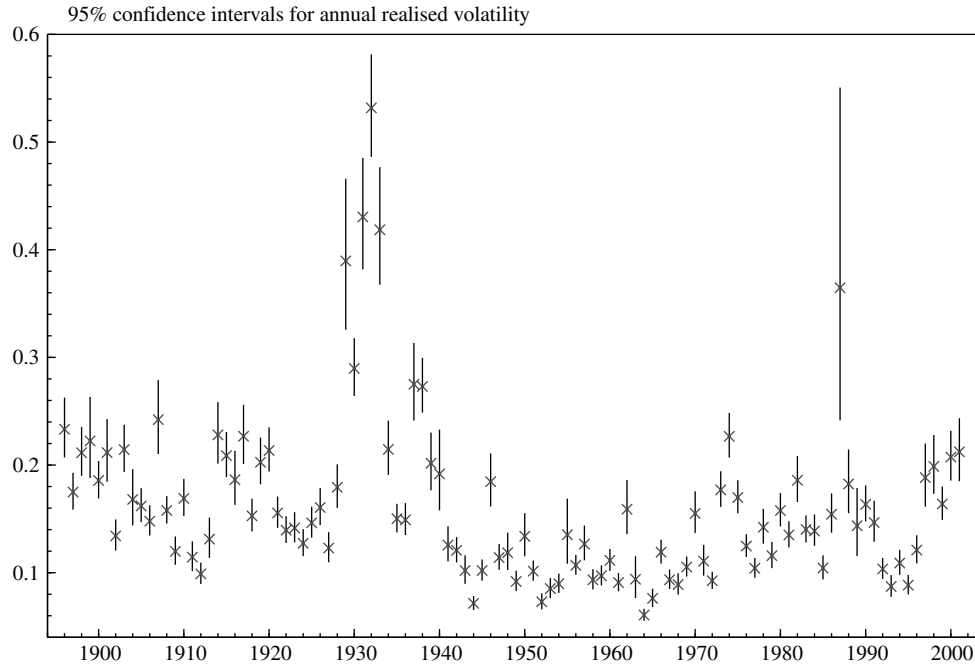
Figure 5. Annual realized volatility \sqrt{\sum_{j=1}^M y_{j,n}^2} for the Dow Jones Industrial Average (marked with crosses) together with 95% confidence intervals. Code: schwert.ox
