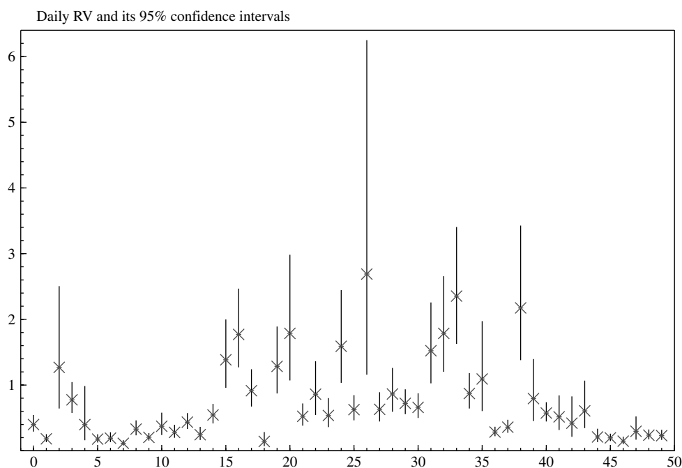
Figure 2. Daily RV, [y_M^*]_i , drawn against n for the first 50 days of the sample. Also drawn as vertical bars are the 95% intervals based on the log transformation. Throughout M = 144 . Code: se.realised.ox
