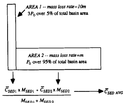
Figure 2. Schematic model of basin having ten-fold higher erosion rate over 5 per cent of area (e.g. mountainous terrain?). Production rate is higher by a factor of three in area of high erosion. Basin area, 10 \text{ km}^2 . See Table II for model data
