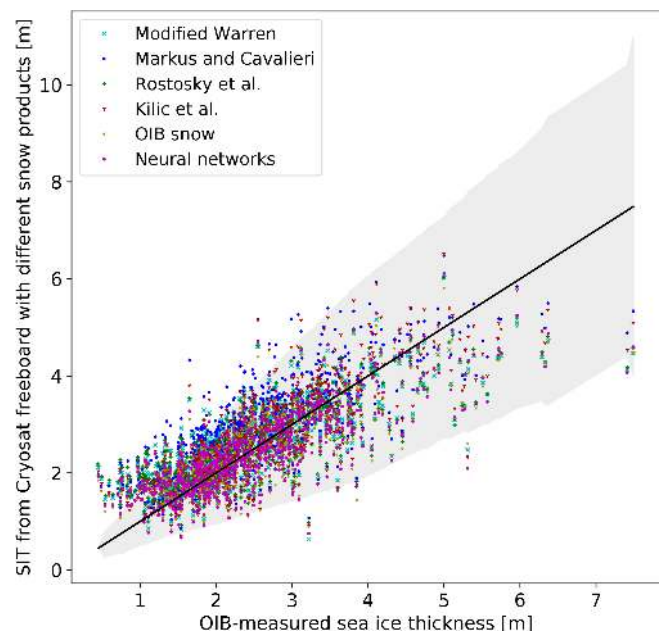
Figure 9. OIB-measured SIT (all data) versus estimated SIT using CryoSat freeboard with different snow depth algorithms.
