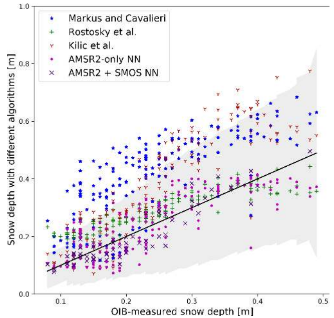
Figure 4. OIB-measured snow depth (test data) versus estimated snow depth using different algorithms. Note that Markus and Cavalieri (1998) should only be applied over FYI, but this plot also includes MYI.
