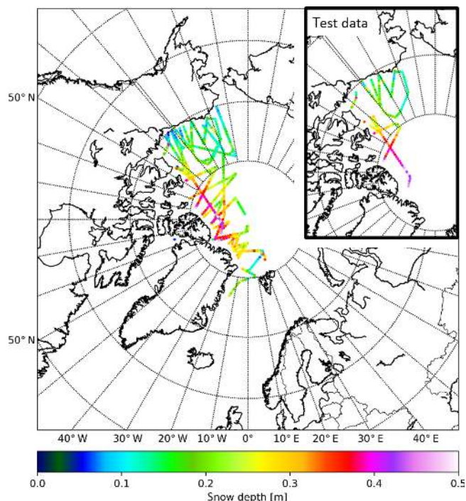
Figure 3. Flight tracks of the Operation Ice Bridge (OIB) campaigns 2013, 2014 and 2015. The measured snow depth is colour-coded. The box on the top right shows which part of the OIB data are used as test data.
