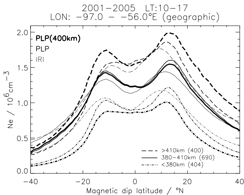
Figure 1. Average day side latitudinal electron density profiles (for Kp < 3 ), as derived from CHAMP PLP (PLP), as predicted by IRI (IRI), and from PLP readings normalized to 400-km altitude (PLP(400 km)). Sampled height ranges are given in the right bottom of the figure, where the total number of CHAMP orbits is also given in brackets.
