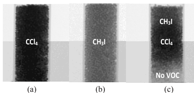
Fig. 9. (a) – CCl 4 adsorption; (b) – CH 3 I adsorption; (c) – co-adsorption of CCl 4 and CH 3 I with roll-up of CH 3 I.
