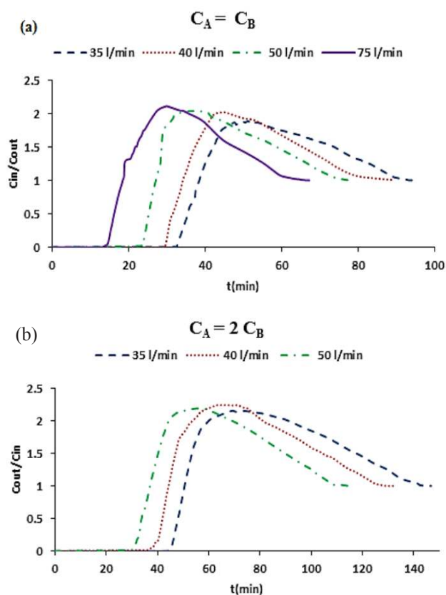
Fig. 10. Qualitative interpretation of binary co-adsorption of organic vapours (A = C 2 H 4 Cl 2 ; B = C 7 H 16 ) showing the influence of the flow rate for (a) equal and (b) different inlet concentrations of the vapours.
