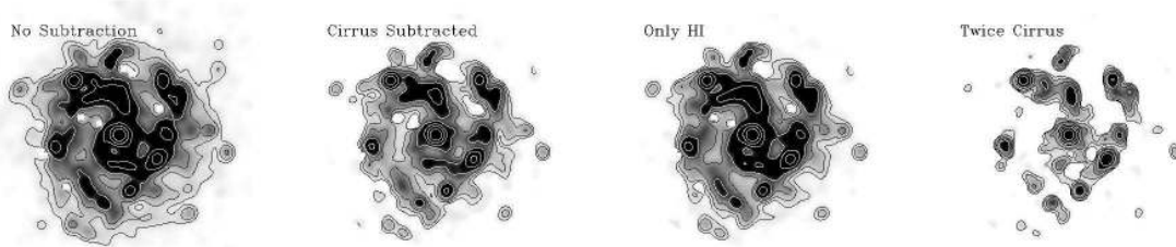
FIG. 5.— Illustration of the cirrus subtraction for NGC 3184. Infrared emission at \lambda = 24\mu\text{m} and 1 kpc resolution. Contours run from 0.1 to 6.4 \text{ MJy sr}^{-1} , stepping by factors of two. Contours \geq 0.8 \text{ MJy sr}^{-1} are white. Individual panels show left to right: no subtraction, 24\mu\text{m} emission after our cirrus subtraction, 24\mu\text{m} emission after our cirrus subtraction applied only for dust associated with H I, and 24\mu\text{m} emission after cirrus subtraction using double the recommended radiation field.
