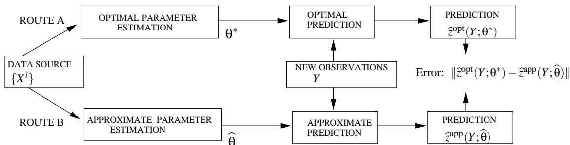
Figure 1: Route A: computationally intractable combination of parameter estimation and prediction. Route B: computationally efficient combination of approximate parameter estimation and prediction.
