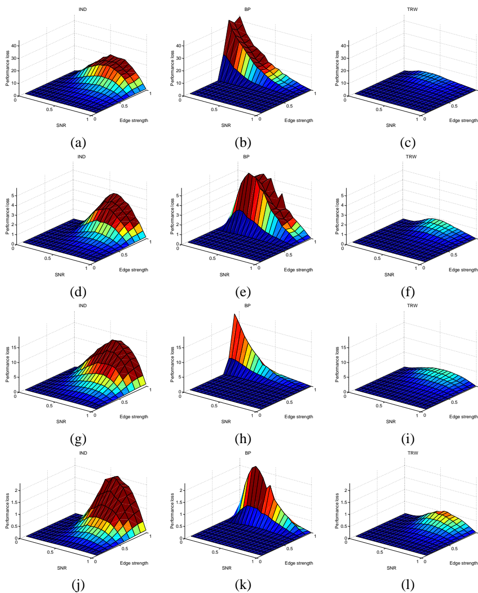
Figure 5: Surface plots of the percentage increase in MSE relative to Bayes optimum for different methods as a function of observation SNR for grids with N = 64 nodes. Left column: independence model (IND). Center column: ordinary belief propagation (BP). Right column: tree-reweighted algorithm (TRW). First row: Attractive coupling and a Gaussian mixture with components (v_0, \sigma_0^2) = (-1, 0.5) and (v_1, \sigma_1^2) = (1, 0.5) . Second row: Attractive coupling and a Gaussian mixture with components (v_0, \sigma_0^2) = (0, 1) and (v_1, \sigma_1^2) = (0, 9) . Third row: Mixed coupling and a Gaussian mixture with components (v_0, \sigma_0^2) = (-1, 0.5) and (v_1, \sigma_1^2) = (1, 0.5) . Fourth row: Mixed coupling and a Gaussian mixture with components (v_0, \sigma_0^2) = (0, 1) and (v_1, \sigma_1^2) = (0, 9) .
