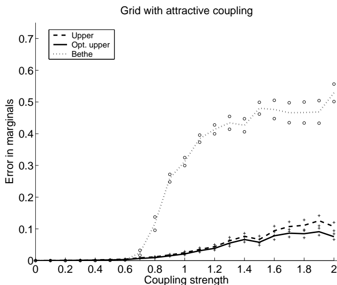
Figure 2: Contrast of the instability of the ordinary sum-product algorithm with the stability of the tree-reweighted version (Wainwright et al., 2005). Results shown with a grid with N = 100 nodes over a range of attractive coupling strengths. The ordinary sum-product undergoes a phase transition, after which the quality of marginal approximations degrades substantially. The tree-reweighted algorithm, shown for two different settings of the edge weights \rho_{st} , remains stable over the full range of coupling strengths. See Wainwright et al. (2005) for full details.
