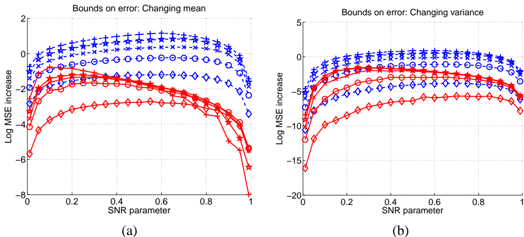
Figure 6: Comparison of actual MSE increase and upper bounds for grid with N = 64 nodes with attractive coupling. (a) Equal variances \sigma_0^2 = \sigma_1^2 = 0.5 , and mean vectors (\mathbf{v}_0, \mathbf{v}_1) ranging from (-0.5, 0.5) to (-2.5, 2.5) . (b) Equal mean vectors \mathbf{v}_0 = \mathbf{v}_1 = 0 , and variances (\sigma_0^2, \sigma_1^2) ranging from (1, 1.25) to (1, 25) .
