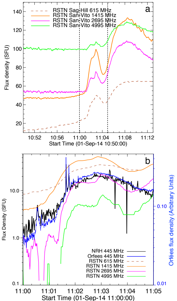
Fig. 6. Panel a: flux densities at 615 MHz from Sagamore Hill site and 1.4, 2.7 and 5.0 GHz from the San-Vito site of the RSTN network. Each of the flux density curves has a steady background which lasts for several hours prior to the event. We used this to perform a background subtraction on each frequency (the rise in flux of 615 and 1415 MHz before the time of interest is taken into account in the flux uncertainty at these frequencies in the analysis below). The dashed lines represent the region of interest (the type IV burst). Panel b: magnification of the RSTN flux density spectrum (between the dashed lines demarcated in (a)) with the NRH and Orféas 445 MHz flux density curve for comparison. The flux densities from all three instruments show a good relationship of flux density variation with time.
