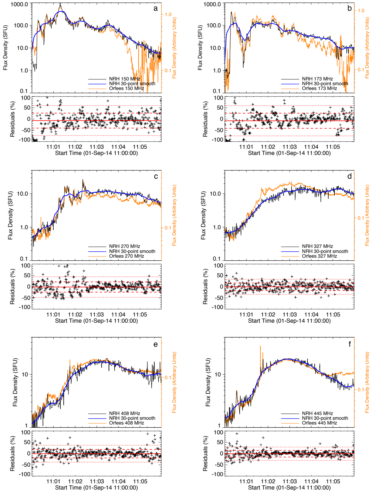
Fig. 5. Flux densities of the large radio source for all NRH frequencies (black; units of SFU) and flux density from Orfées at the same frequency (orange; arbitrary units). The blue line is a 30-point box-car smooth of the NRH time profiles. The difference between the black and blue curves provides the residuals over time for each panel. Residuals larger than 2\sigma are indicative of sporadic radio bursts. The 150–173 MHz sources have much larger flux densities and are also more bursty in nature (larger residual spread). At 228 MHz and above the flux densities are much weaker, while at 300 MHz and above the flux is weaker and much more smoothly varying in time, that is, the residuals mainly varying by less than 2\sigma , indicative of flux variation due Gaussian noise only (very few sporadic radio bursts) above these frequencies.
