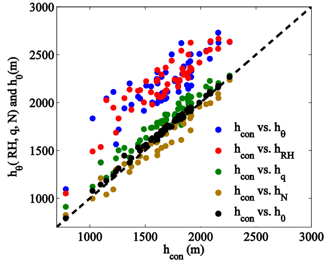
Figure 6. Comparison of the climatological h_{con} with h_{\theta} (blue), h_{RH} (red), h_q (green), h_N (brown) and h_0 (black) for the period 1998–2008.
