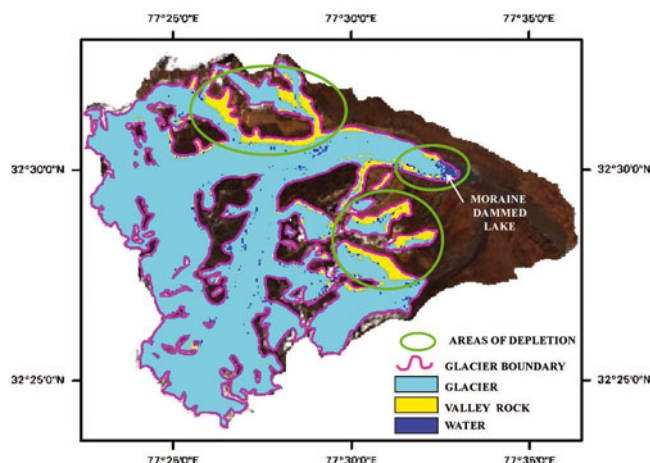
Fig. 6. Comparative assessment of the glacier area obtained from AWiFS (2004) and the glacier boundary derived from SOI toposheets (1963). The false-colour composite (red: B4, green: B3, blue: B2) is from the AWiFS image. All the glacier-cover classes (snow, ice, MID, debris) have been merged into a single class: glacier. Note the presence of valley-rock and water within the glacier area, indicating glacier depletion and recession (circled in green).
