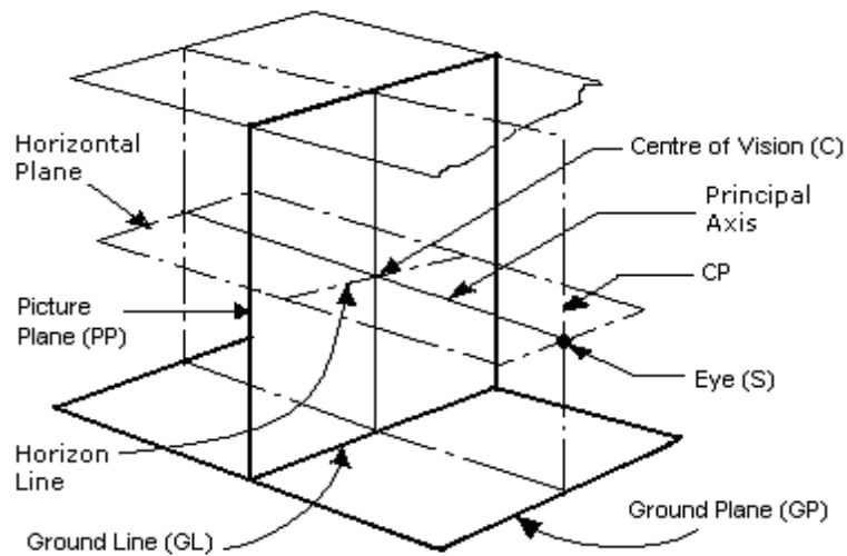
Fig. 2.3: Perspective view planes and points, which are important to be noticed.
