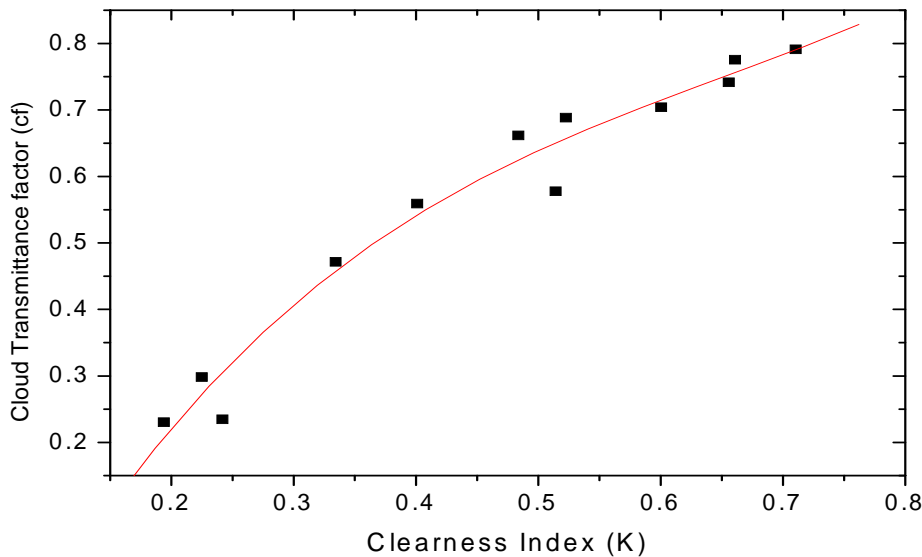
Figure 3. Correlation coefficient in between clearness index K and cloud transmittance factor (cf) at Lukla in 2009-2010.
