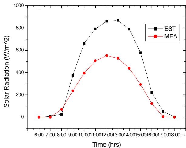
Figure 2. Diurnal Variation of global solar radiation in clear sky day on 26 January, 2010 at Lukla.
