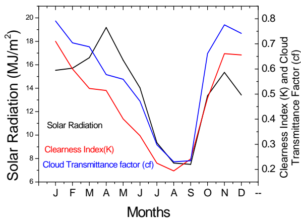
Figure 4. Relationship between global solar radiation, clearness index and cloud transmittance factor at Lukla in 2009-2010.
