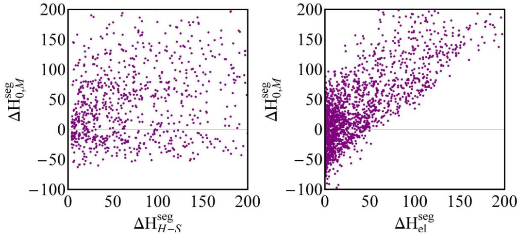
FIG. 3 A comparison of our segregation model, \Delta H_{0,M}^{seg} , with the Hondros-Seah model ( \Delta H_{H-S}^{seg} ) and elastic-only enthalpy ( \Delta H_{el}^{seg} ).
