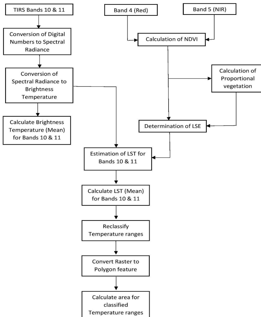
Fig – 2: Flowchart
