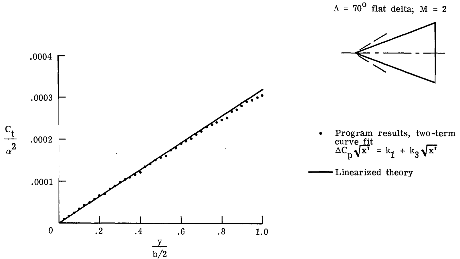
Figure 11.- Program thrust distribution for a flat wing treated as if it were a cambered wing.
