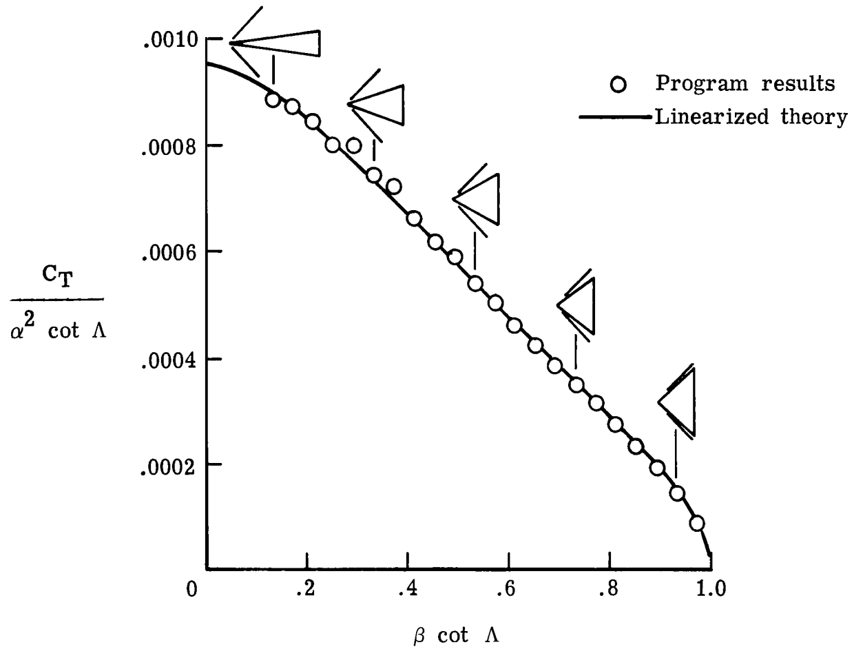
Figure 8.- Comparison of program and theoretical thrust coefficients for a series of flat delta wings.
