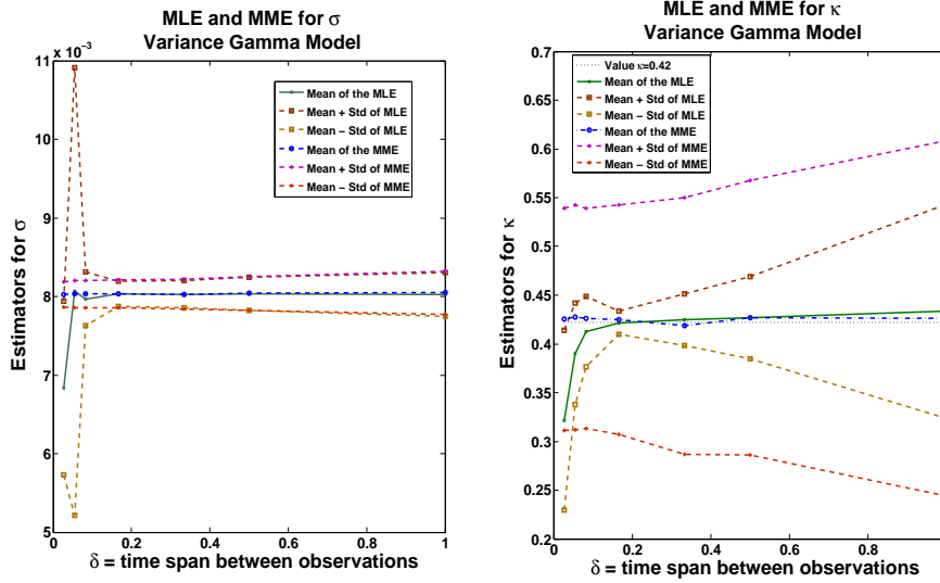
FIG 1. Sampling mean and standard error of the MME and MLE for the parameters \sigma and \kappa based on 100 simulations of the VG model with values T = 252 \times 3 , \sigma = \sqrt{6.447 \times 10^{-5}} = .0080 ; \kappa = 0.422 ; \theta = -1.5 \times 10^{-4} ; b = 2.5750 \times 10^{-4} .
