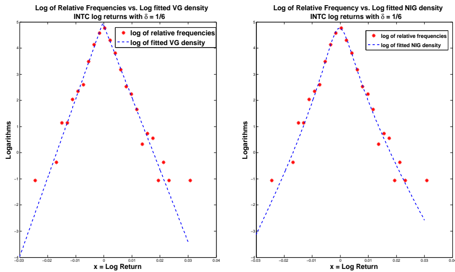
FIG 8. Logarithm of the histograms of INTC returns for \delta = 1/6 and the fitted VG and NIG models using Maximum Likelihood Estimation.
