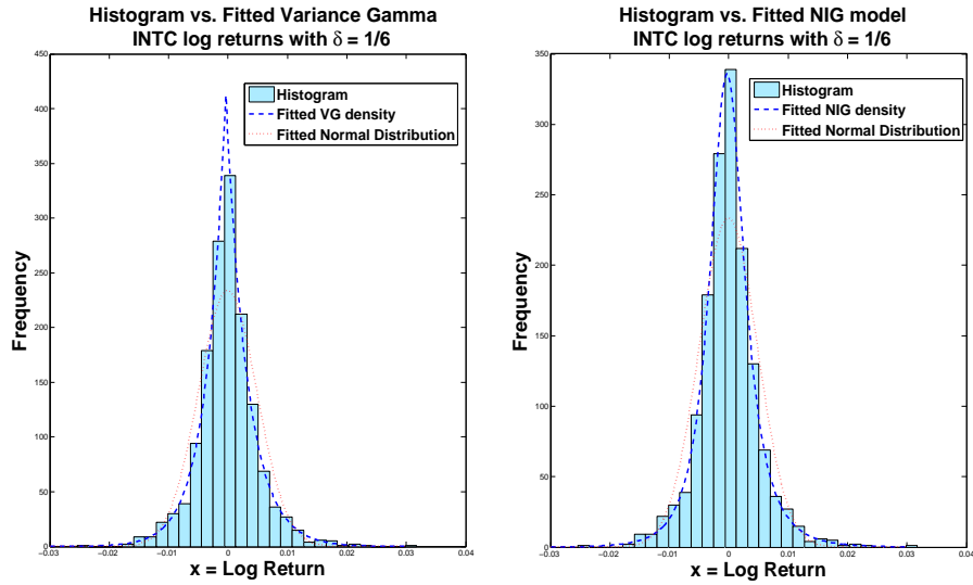
FIG 7. Histograms of INTC returns for \delta = 1/6 and the fitted VG and NIG models using Maximum Likelihood Estimation.
