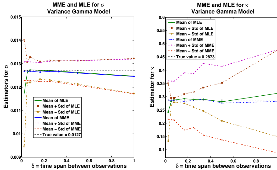
FIG 2. Sampling mean and standard error of the MME and MLE for the parameters \sigma and \kappa based on 200 simulations with values T = 252 , \sigma = .0127 ; \kappa = 0.2873 ; \theta = 1.3 \times 10^{-3} ; b = -1.7 \times 10^{-3} .
