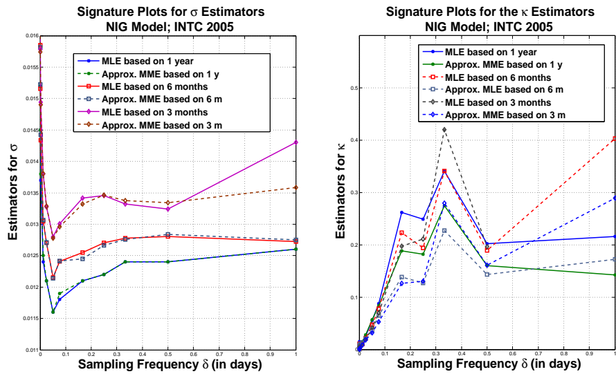
FIG 6. Signature plots for the MLE and MME for \sigma under a NIG model based on different time horizons.
