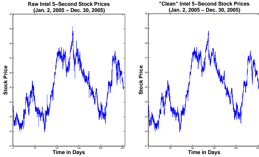
FIG 5. Intel stock prices during 2005 before and after preprocessing.
