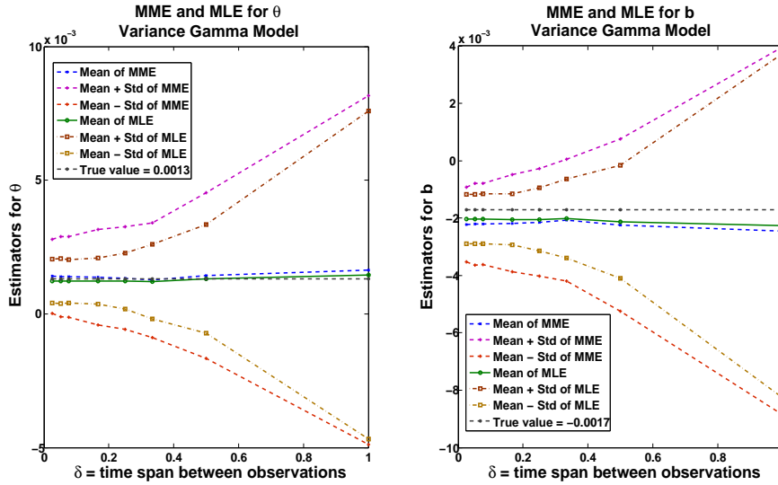
FIG 3. Sampling mean and standard error of the MME and MLE for the parameters \theta and b based on 200 simulations with values T = 252 , \sigma = .0127 ; \kappa = 0.2873 ; \theta = 1.3 * 10^{-3} ; b = -1.7 * 10^{-3} .
