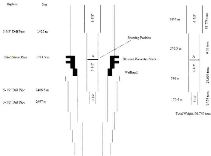
Fig. 9. Examined well configuration
