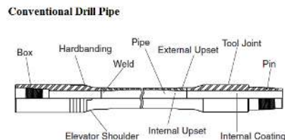
Fig. 2. Drill pipe tool joint
