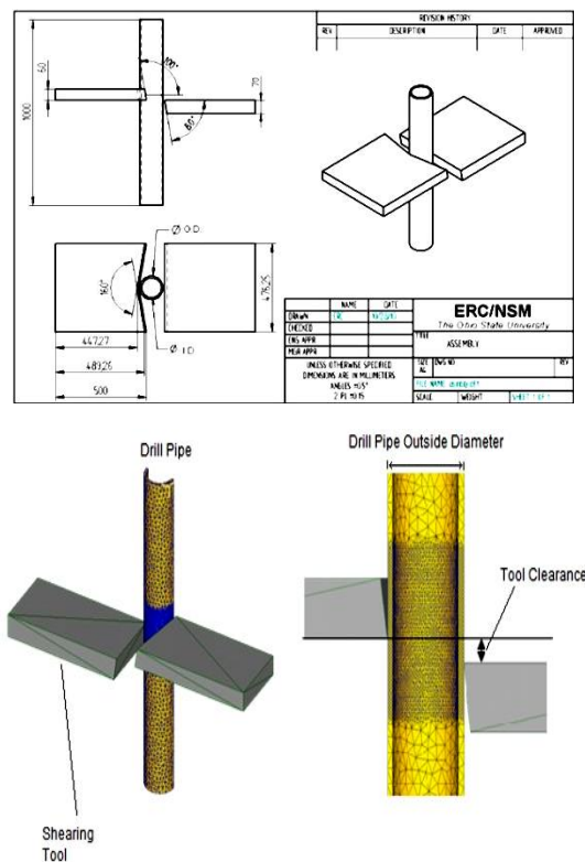
Fig. 3. The geometries of shear ram and drill pipe
