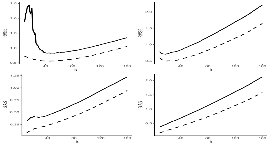
Figure 5: Root MSE estimates (top panels) and Bias estimates (bottom panels) of \widehat{\text{XMES}}^*/\text{XMES} (solid line) and \widehat{\text{XMES}}^*/\text{XMES} (dashed line), as functions of k , for the bivariate t_3 and t_5 -distributions on (0, \infty)^2 , respectively, from left to right.
