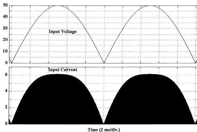
Fig. 7. Input voltage and current in PFC application.
