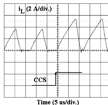
Fig. 9. Inductor current transient response to a step up change in CCS.
