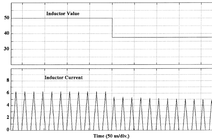
Fig. 5. Simulation results of the open loop response to a 25% step change of the inductor value.
