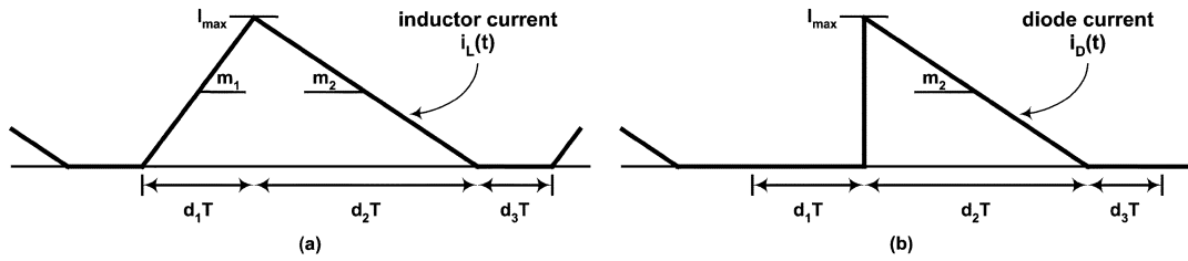
Fig. 2. Typical current waveforms of (a) inductor and (b) diode operating in DCM.
