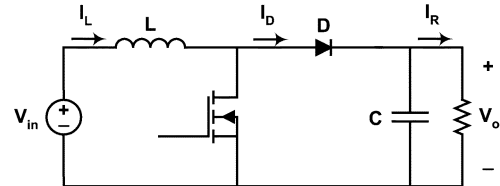
Fig. 1. Boost converter.
