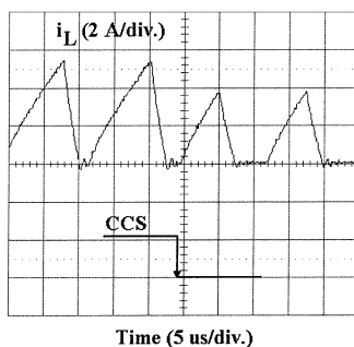
Fig. 8. Inductor current transient response to a step down change in CCS.
