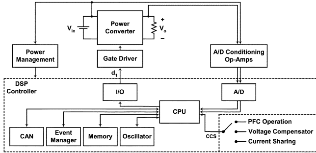
Fig. 3. Block diagram of the digital current controller.
