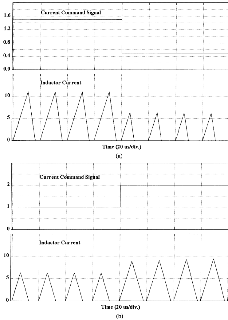
Fig. 4. Simulation results of the converter transient response to a step change in the current command signal: (a) step down and (b) step up.
