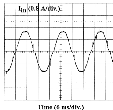
Fig. 10. Input current of the PFC converter after being filtered by the EMI filter.
