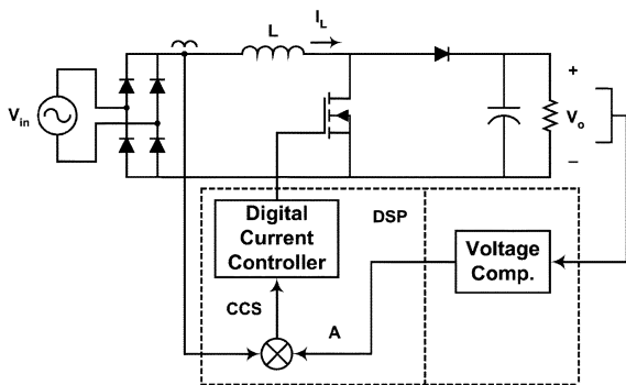
Fig. 6. Block diagram of the PFC converter.
