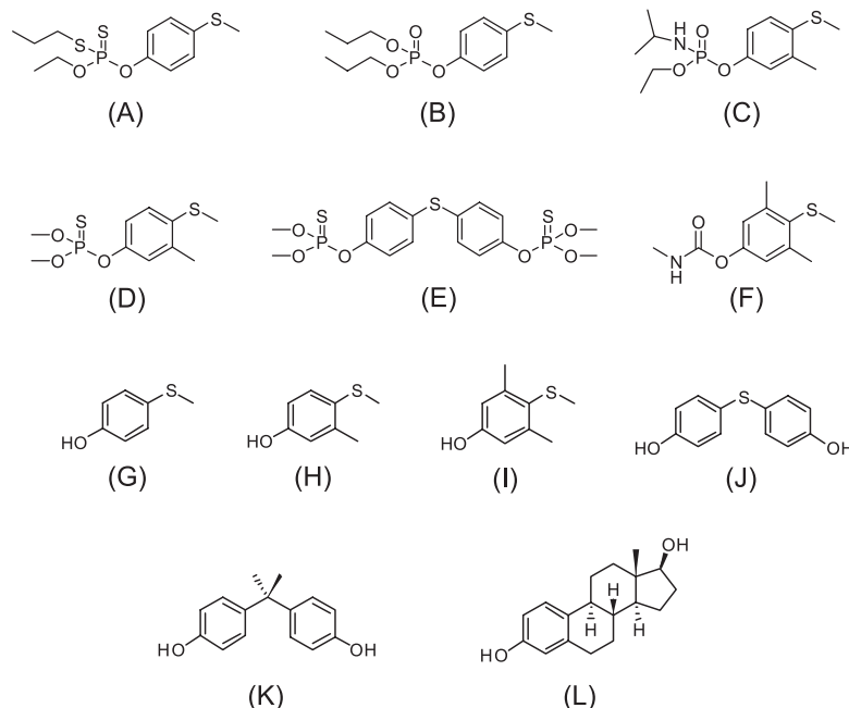
Fig. 1. Chemical Structure of the Test Compounds
