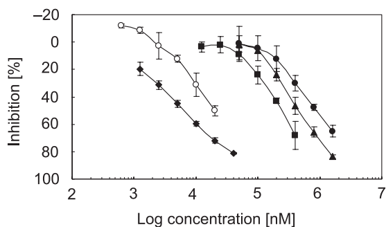
Fig. 3. Dose-response Curves in ER-ELISA ●; MTP, ▲; MMP, ■; DMP, ◆; TDP, ○; BPA (reference compounds). Each point represents the mean of triplicate.
