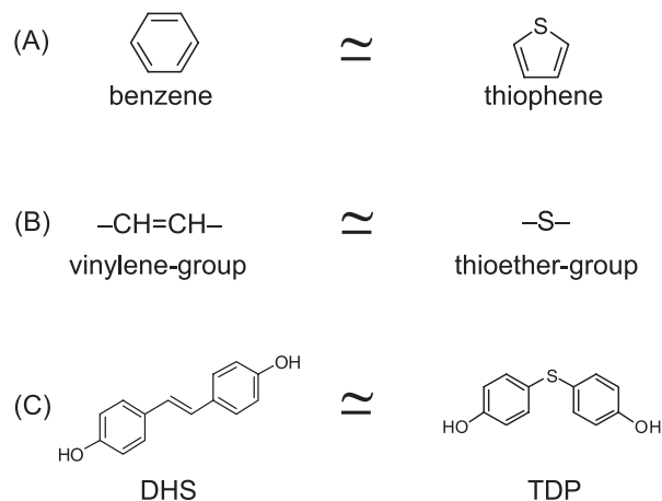
Fig. 4. Bioisosteric Relationships between Benzene and Thiophene (A), Vinylene-group and Thioether-group (B), and 4,4'-Dihydroxystilbene (DHS) and TDP (C)
