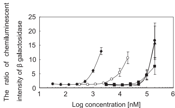
Fig. 2. Dose-response Curves in Yeast Two-hybrid Assay ●; MTP, ▲; MMP, ■; DMP, ◆; TDP, ○; BPA (reference compounds). Each point represents the mean of triplicate.
