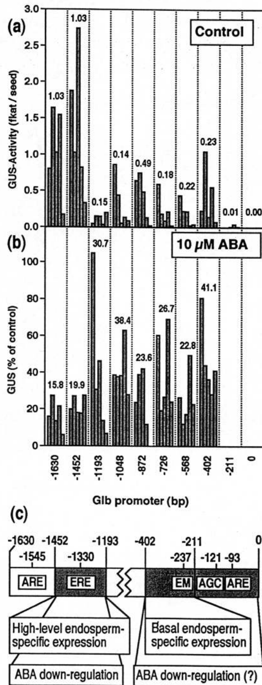
Figure 3 Deletion analysis of the the Glb promoter in germinating Havana 425 tobacco seeds. (a) GUS activity (fkat/seed) of control seeds. (b) Down-regulation by 10 \mu M ABA expressed as % GUS activity relative to the corresponding control populations of seeds shown in (a). Seeds of a Glb-GUS promoter deletion series with 5 independent transformants for each deletion were imbibed in continuous light with and without 10 \mu M ABA. Extracts were prepared from seeds after 3 days when ca. 70 % of controls and none of ABA treated seeds had ruptured endosperms. The extracts were assayed for GUS activity. For each construct, bars in the same relative position represent seed of the same independent transformant shown in the order: 2 high-, 2 medium-, and 1 low-expressing line as judged from tests of the transformants described by Vögeli-Lange et al. [44]. Each bar represents the mean value, usually of replicate assays, in two independent experiments. The numbers above the bars are the median value obtained with each deletion. (c) Diagram illustrating regions of the Glb promoter relevant to regulation in germinating seeds. Filled boxes: The distal region (-1452 to -1193) important for high-level expression and ABA down-regulation; the proximal region -402 to -211 necessary and sufficient for low-level expression in the micropylar endosperm; and, the proximal region downstream of -402 that may also contribute to ABA down-regulation. Symbols: ARE, an ABA-responsive element (TAACAAA) important for down-regulation by ABA of \alpha -amylase genes in barley endosperm [15]; AGC, one copy in inverse orientation of the AGC box (AGCCGCC) present as two copies (-1346 and -1314) in the ERE [16]; EM, an EM box (TGTAAG) important for endosperm-specific expression of cereal storage-protein genes in tobacco [4]; and, ERE, the Glb ethylene-responsive element [30]. Numbers refer to position relative to the start of transcription.
