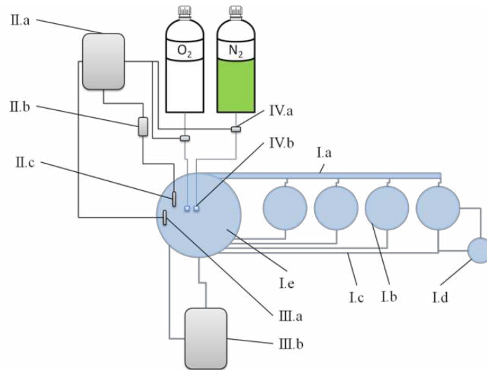
Fig. 31. Exposure system for oxygen challenge in experiments with juveniles. I.a: supply circuit; I.b: experimental tank; I.c: feedback circuit; I.d: regulation tank for control condition; I.e: water-tower. II.a: control and recorder units; II.b: oxymeter; II.c: oxygen probe. III.a: thermistor; III.b: chiller. IV.a: electrovalve; IV.b: diffusor.
