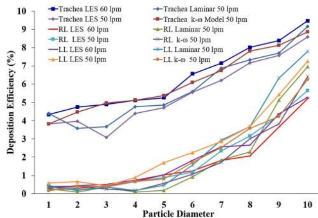
Figure 10. Polydisperse particle DE in different region of the realistic lung model at 50 lpm and 60 lpm.
