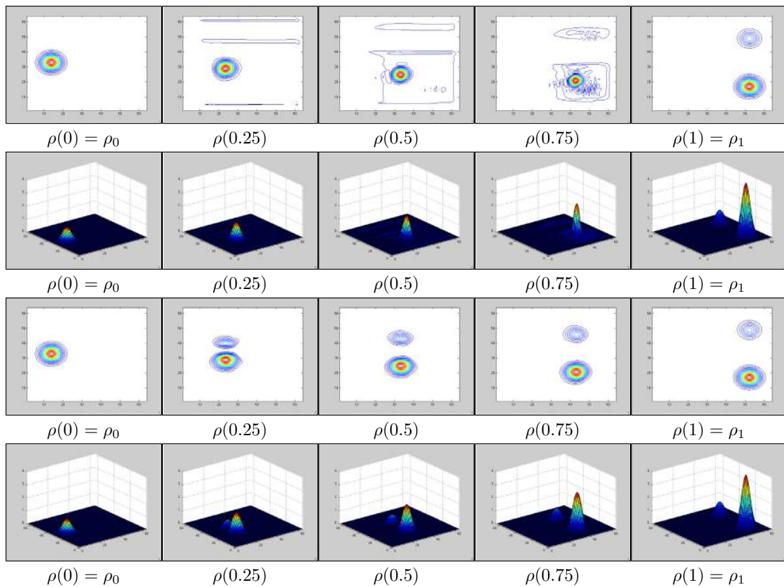
FIGURE 5. Plot of the isovels of the density \rho(t) along the optimal path between two densities of different mass. Top rows : original Benamou–Brenier’s Algorithm, with top and side views; Bottom rows : our algorithm with exponential source term.
