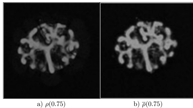
FIGURE 18. Comparison between the interpolation at time t = 0.75 , (a), obtained by solving optimal transport between images (1 – 5) and the original image in grey scale (b).
