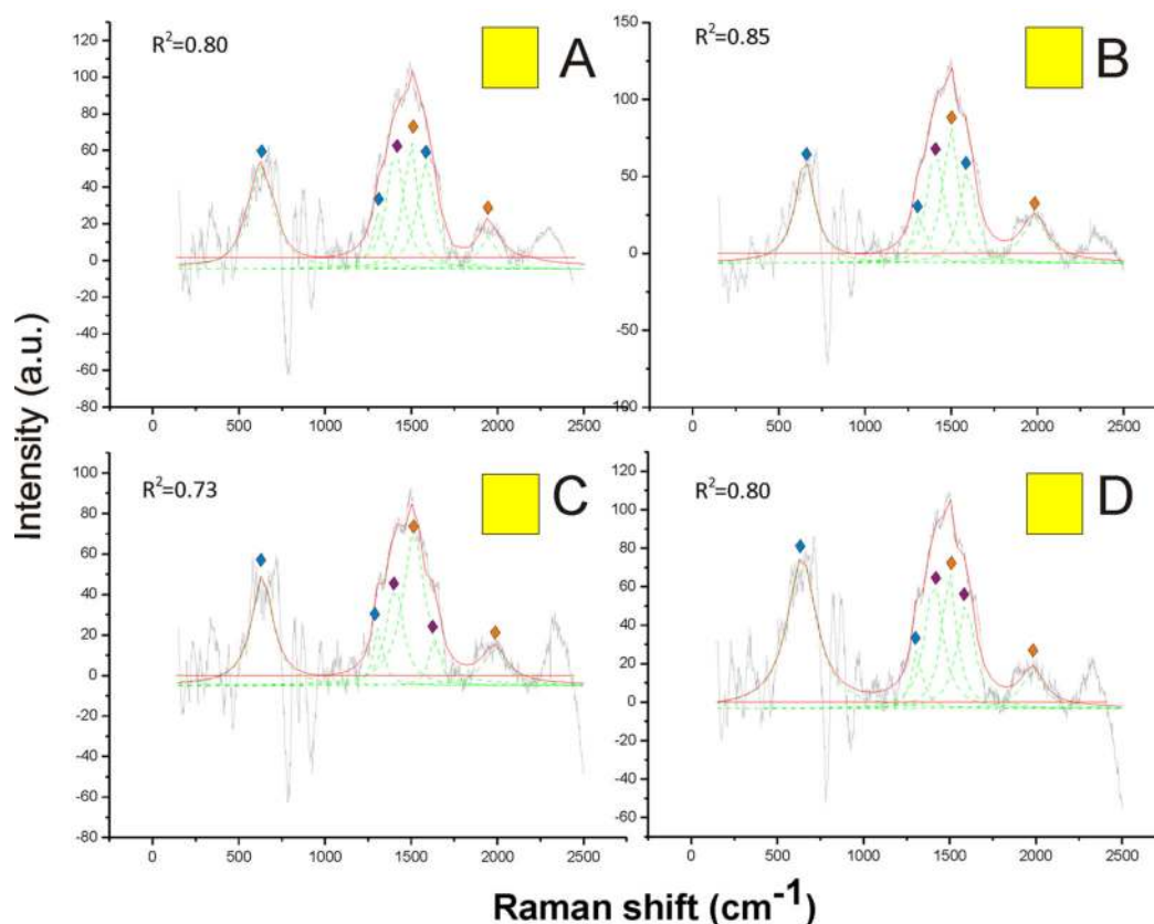
Figure 4 Examples of Raman spectra of yellow hair in Bombus , and peak identification after having applied the reference deconvolution method. The gray line represents the Raman spectrum, the dashed green lines represent the single deconvoluted curves, which highlight the different peaks contributing to the spectrum, and the red line represents the sum of the deconvoluted curves (i.e., the adjustment to the spectrum, whose goodness of fit expressed as R^2 value). ♦ Signature peaks for pheomelanin, ◆ signature peaks for chitin, ◆ signature peaks for N -acetyl-D-glucosamine. (A) Abdomen of Bombus soroeensis ; (B) abdomen of Bombus terrestris ; (C) thorax of Bombus lucorum ; (D) thorax of Bombus monticola .
