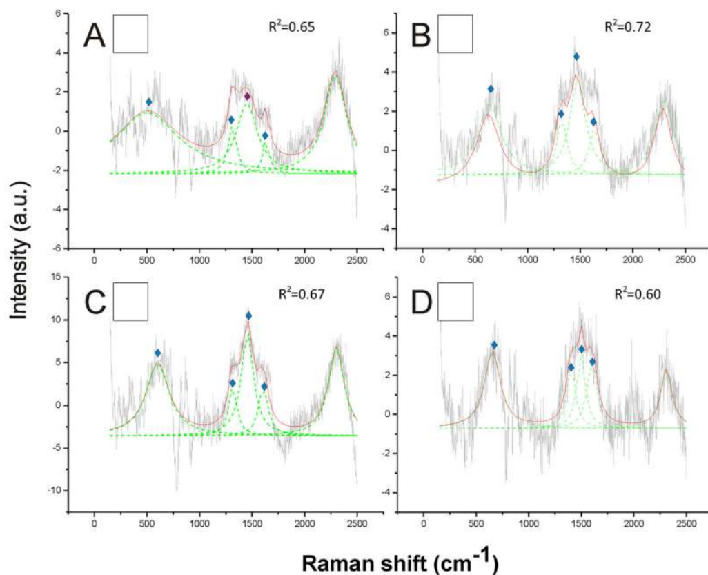
Figure 3 Examples of Raman spectra of white hair, and of hairless thorax ventral side cuticle, in Bombus , and peak identification after having applied the reference deconvolution method. The gray line represents the Raman spectrum, the dashed green lines represent the single deconvoluted curves, which highlight the different peaks contributing to the spectrum, and the red line represents the sum of the deconvoluted curves (i.e., the adjustment to the spectrum, whose goodness of fit expressed as R^2 value). ♦ Signature peaks for chitin, ♦ signature peaks for N -acetyl- D -glucosamine. (A) abdomen of Bombus lucorum ; (B) abdomen of Bombus terrestris ; (C) abdomen of Bombus soroensis ; (D) abdomen of Bombus gerstaeckeri . Note that no melanin peaks and overall very low intensity signal were detected in white hair.
