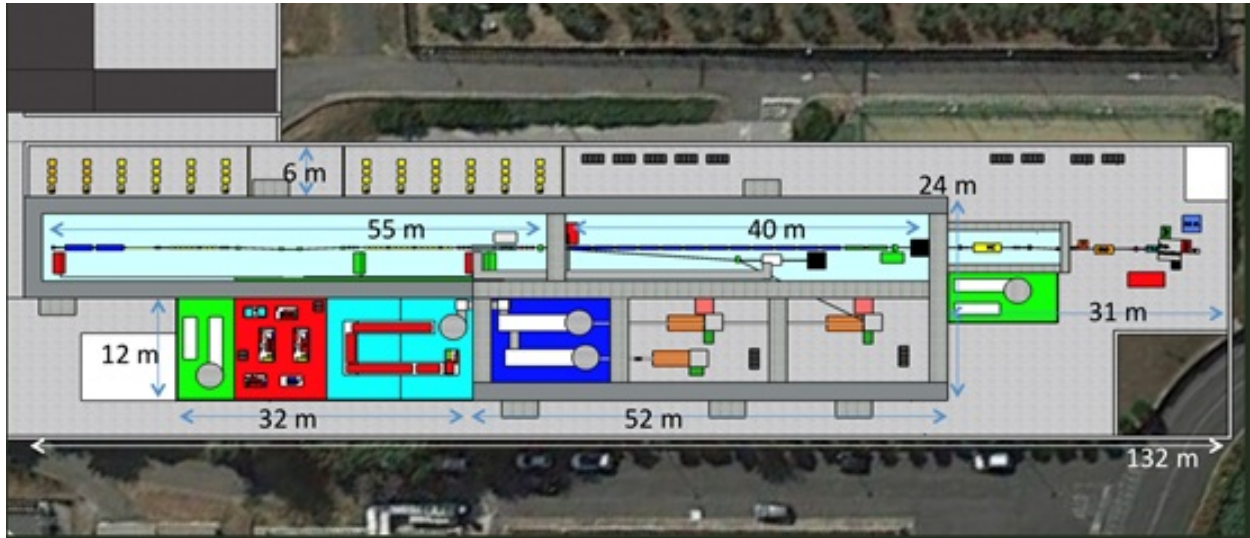
Figure 1: The layout of the EuPRAXIA@SPARC_LAB infrastructure
