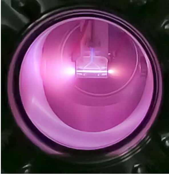
Figure 2: Discharge capillary installed in the SPARC_LAB beamline
