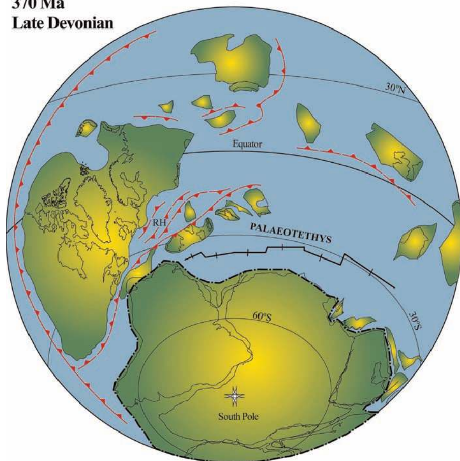
Fig. 10. Late Devonian (Famennian, 370 Ma) reconstruction, modified from Torsvik & Cocks (2004, fig. 6). Symbols as in Figure 2; terrane names as in Figure 9. The Rheno-Hercynian (RH) Terrane was in the process of amalgamation with Laurussia at this time.
