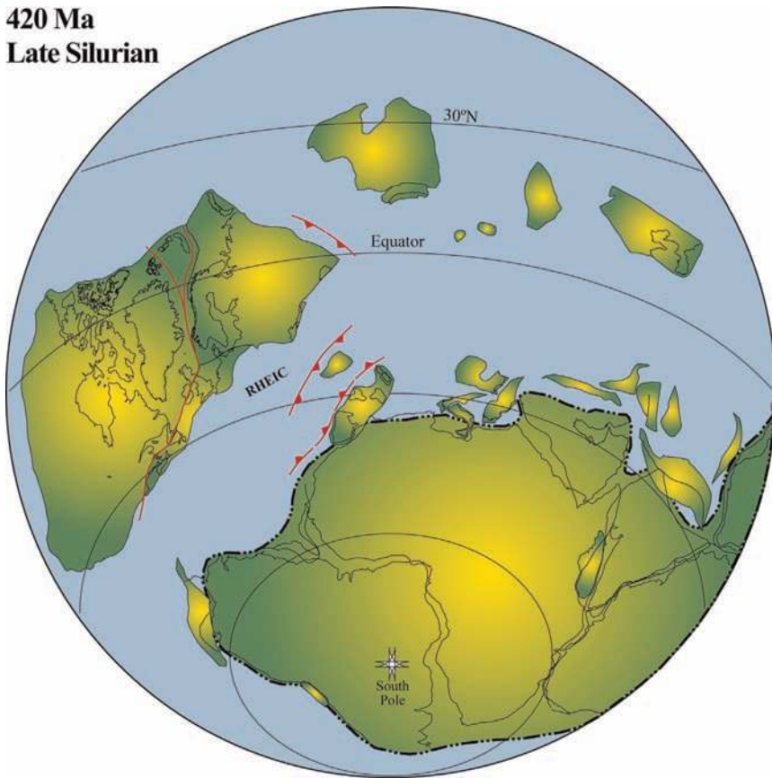
Fig. 8. Late Silurian (Ludlow–Prídolí, 420 Ma) reconstruction, modified from Cocks & Torsvik (2002, fig. 8). Symbols as in Figure 2; terrane names as in Figures 2 and 9. Figures 8–10 are Schmidt’s Equal Area Projection, with projection centre at 30°S.
