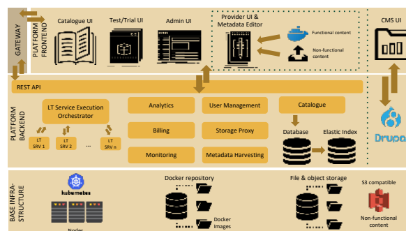
Figure 2: Technical architecture
