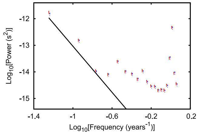
Figure 9. (Top) 95 percent upper limits from an unparameterized power spectrum analysis for a correlated GWB (red points), and uncorrelated common red noise process (blue points) for the six pulsar data set described in Section 4 obtained while varying the intrinsic noise parameters for each pulsar. The upper limit obtained from a power-law analysis of the GWB at a spectral index of 13/3 of 3 \times 10^{-15} is overplotted as a straight line. Frequencies were included from 1/T up to 20/T , with T = 17.66 yr. Beyond these frequencies, the data provides increasingly poorer constraints on a steep red noise process, and so we do not consider higher frequency terms in our model. Both the correlated and uncorrelated power spectrum are completely consistent with one another at all frequencies. The difference in the log evidence between the correlated and uncorrelated models was 0.2 \pm 0.3 , indicating no support for the presence of a correlated signal in the data set.
