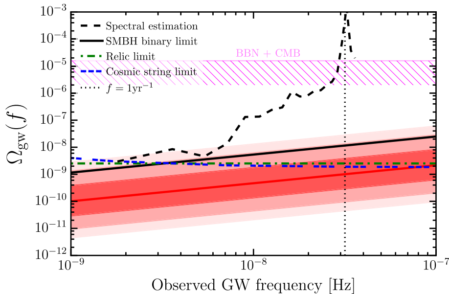
Figure 1. Summary of key results from the analysis of a six pulsar data set from the 2015 EPTA data release (D15). Results are presented in terms of \Omega_{\text{gw}}(f) as a function of GW frequency, with H_0 = 70 \text{ km s}^{-1} \text{ Mpc}^{-1} . We indicate the 95 per cent upper limits on the amplitude of a correlated GWB assuming a power-law model with a spectral index of \gamma = 13/3 (solid black line; Section 5) and for a more general analysis, where the power is determined simultaneously at a set of discrete frequencies (dashed line), as discussed in Section 5.1.1. The red shaded areas represent the central 68 per cent, 95 per cent, and 99.7 per cent confidence interval of the predicted GWB amplitude according to Sesana (2013b) under the assumptions that an SMBHB evolves purely due to gravitational radiation reaction and binaries are circular (see Section 6.1 for more details). Only about 5 per cent of the distribution is excluded, meaning that our limit does not place significant restrictions on the cosmic SMBHB population. We also indicate 95 per cent upper limits obtained for a stochastic relic background (green dash-dotted line; Section 6.3), and for cosmic string network backgrounds (blue triple-dashed line; Section 6.2). The cosmic string limit plotted corresponds to a fiducial model for a population of cosmic strings, with the following parameters: string tension G\mu/c^2 = 10^{-7} , the birth-scale of loops relative to the horizon \alpha_{\text{cs}} = 1.6 \times 10^{-6} , spectral index q = 4/3 , cut-off on the number of emission harmonics n_* = 1 , and intercommutation probability p = 1 . Finally, we indicate recent constraints placed by CMB (Sendra & Smith 2012), and BBN (Allen 1997; Maggiore 2000; Planck Collaboration XIII 2015) observations.
