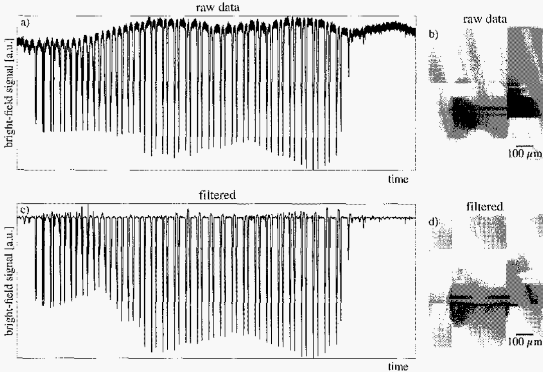
Fig. 2. Large area scans of a region showing high-powered UV laser damage, raw and filtered data reconstructions. Without filtering (a, b), fluctuations in the illumination flux level can appear as large-scale changes in the apparent reflectivity that follow the direction of the scanning path, slightly inclined from vertical. Intensity-level filtering (c, d) is most effective in regions surrounded by open mask areas. In this example, the largest reflectivity change occurs in the dark regions, where the reflectivity falls to 31% of the background level.
