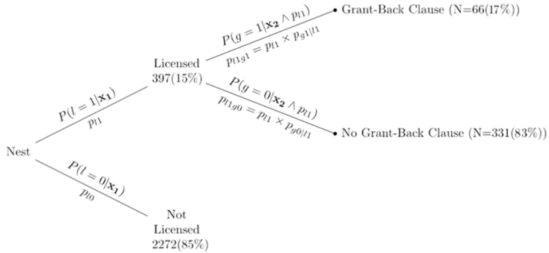
Figure 1: The Hierarchical Nested Tree Structure
