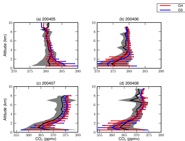
Fig. 6. Observed and GEOS-Chem a posteriori model CO 2 vertical profiles (ppm) taken from the CO 2 Budget and Regional Airborne Study over the eastern North America averaged over (a) May, (b) June, (c) July, and (d) August 2004. The GEOS-Chem model, described at a horizontal resolution of 2° × 2.5°, has been sampled at the time and location of each measurement. Data and model concentrations have been averaged over 500 m intervals. Monthly mean observations are denoted by the black lines, with the grey envelope representing the 1-standard deviation about that mean. Blue and red lines denote the monthly mean CO 2 concentrations corresponding to the G4 and G5 a posteriori flux estimates, respectively. The horizontal lines about a posteriori concentrations denote the 1-standard deviation about the monthly mean.
