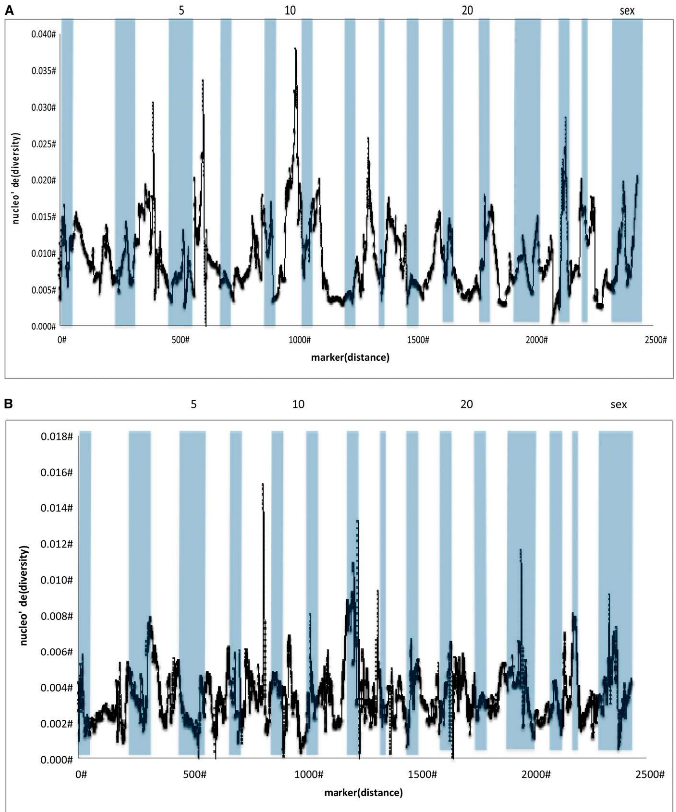
Figure 4 Nucleotide diversity as calculated by Watterson's theta in markers that mapped to two linkage maps of the O. mykiss genome (Miller et al. 2012; Hecht et al. 2012). The kernel-smoothed average for all markers that mapped is presented for (A) Sashin Creek migrants and (B) Little Sheep Creek samples. Chromosomes are alternately shaded with some chromosomes labeled.
