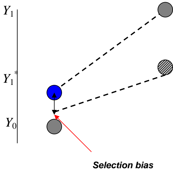
Figure 3: Bias in double-difference estimates for a targeted anti-poverty program
