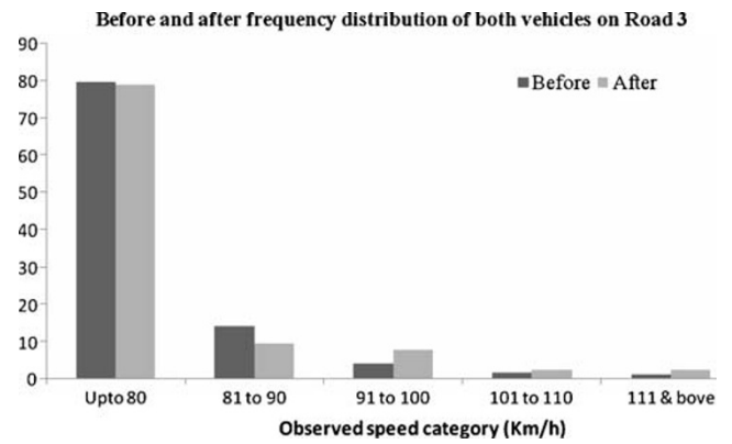
Fig. 3 Comparison between before and after frequency distribution of both vehicles on Road 3 for various observed speed categories
