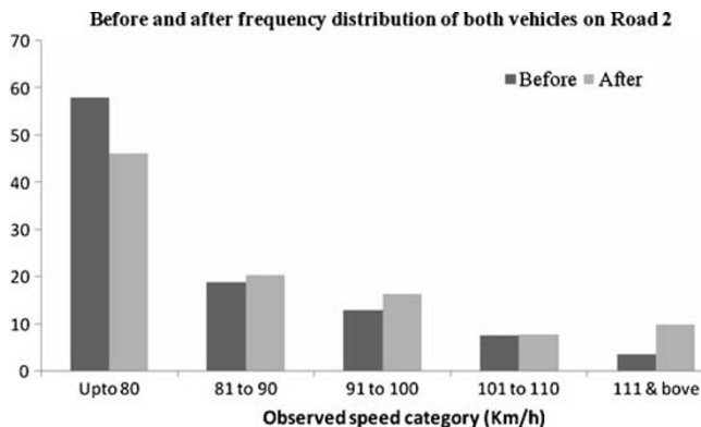
Fig. 2 Comparison between before and after frequency distribution of both vehicles on Road 2 for various observed speed categories
