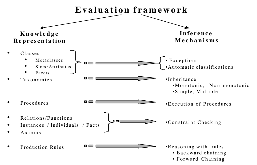
Figure 1. Evaluation framework.
