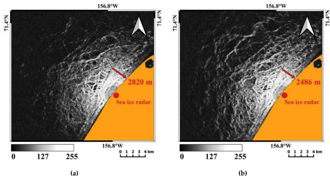
Figure 2. Coastal radar images taken on 13 Jan 2012, 03:18 UTC (a) and 24 Jan 2012, 03:18 UTC (b). Images indicate compression towards the coast during the time period spanned by the two dates. Red arrows indicate one example where a ridge has been displaced towards the coast. Land is masked out in orange.
