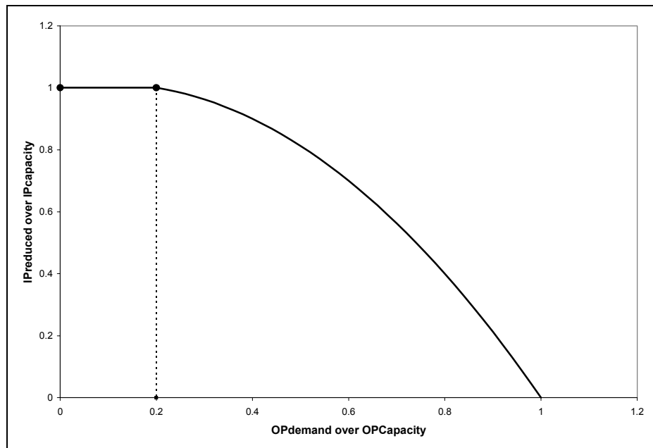
Figure B.16. Effect of OP on IP revised.
