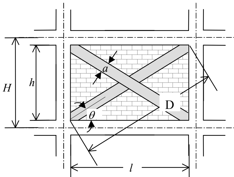
Figure 3. Strut geometry.
