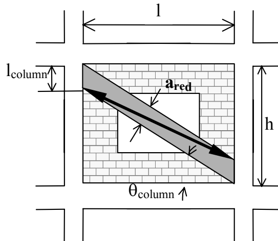
Figure 6. Perforated panel.
