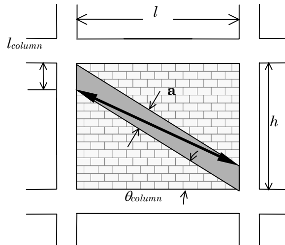
Figure 4. Placement of strut.
