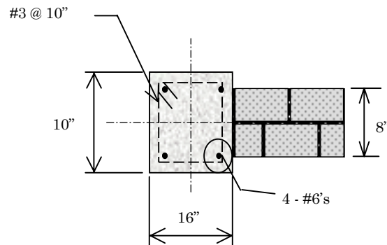
Figure A.4. Column cross-section.
