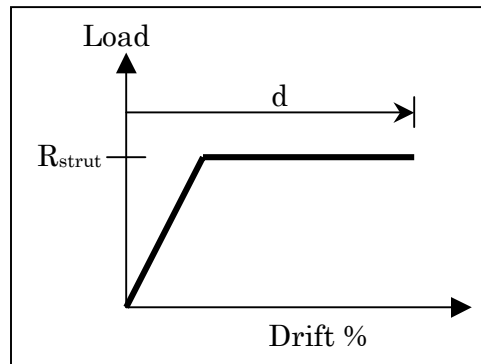
Figure 10. Load-deformation behavior.
