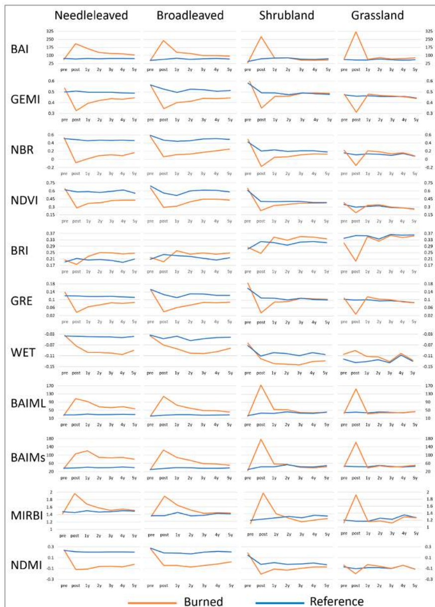
Figure 5. Temporal trajectories for 11 spectral indices in four major vegetation types in northwest Yunnan.
