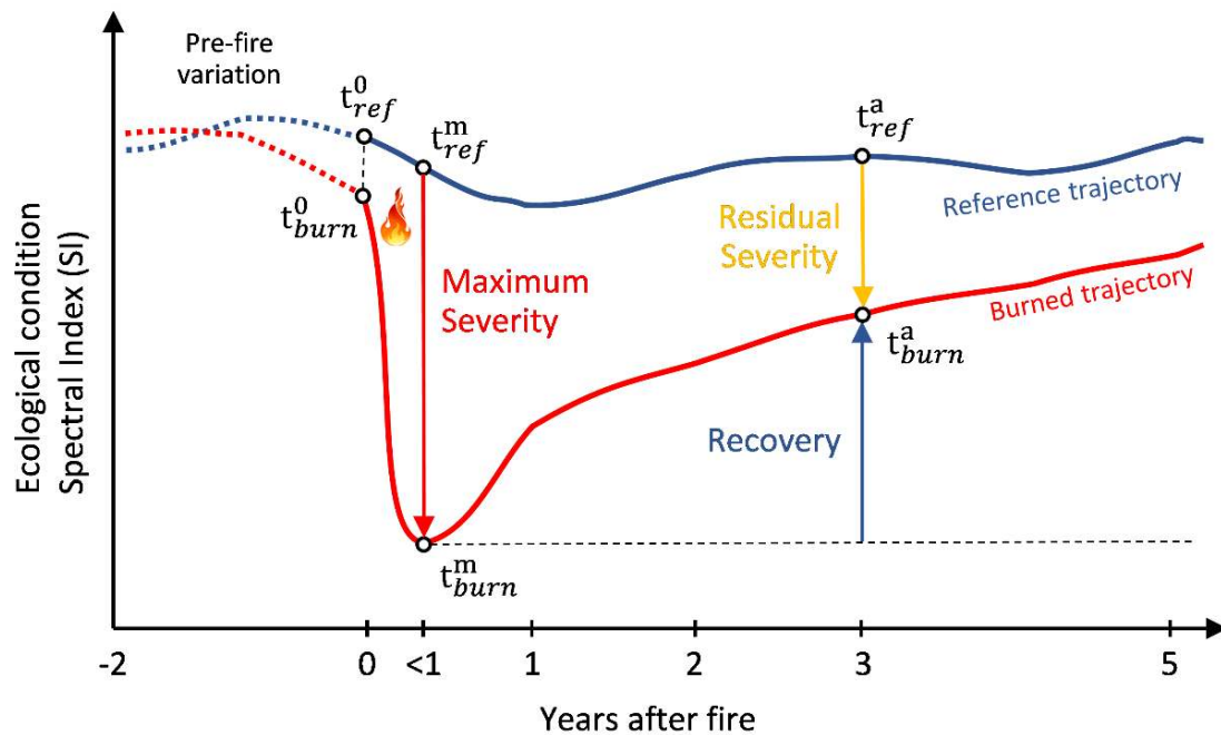
Figure 2. Temporal trajectories of burned and unburned vegetation. This conceptual model represents the effect of fire on vegetation as well as severity and recovery patterns. Spectral Indices serve as proxies to represent the ecological condition of the vegetation. Modified and adapted from Key [65] and Chompuchan Lin [64].
