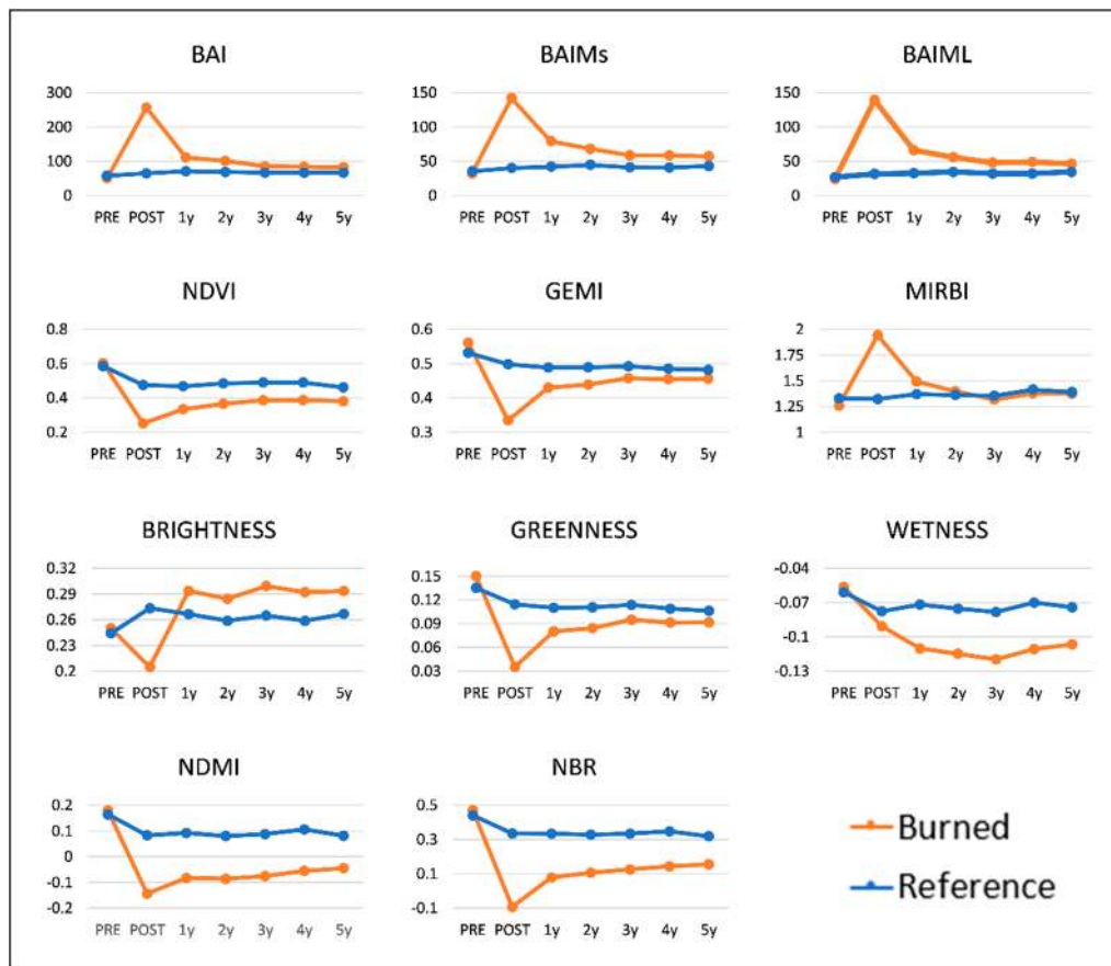
Figure 4. Spectral Indices' trajectories over time: pre- and post-fire, and 1, 2, 3, 4, and 5 years following the fire. The plots represent the SI mean values for the burned and the reference samples of the whole dataset.
