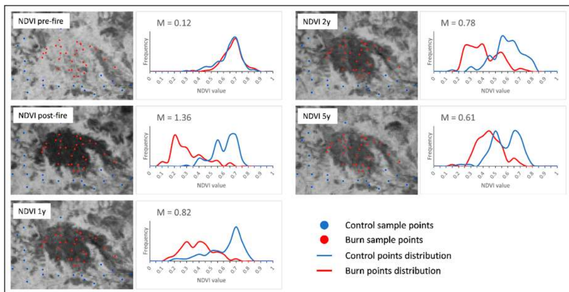
Figure 3. Burned vs. unburned class distributions for the NDVI at pre-fire, post-fire, and 1, 2, 5 years after fire. An example of burn scar, burn and control sample points, as well as the M -statistic results are illustrated.
