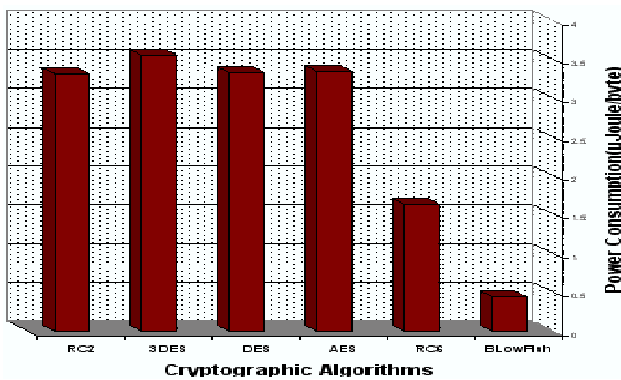
Figure 10: Power consumption for encrypting different audio files in \mu\text{Joule}/\text{Byte}
