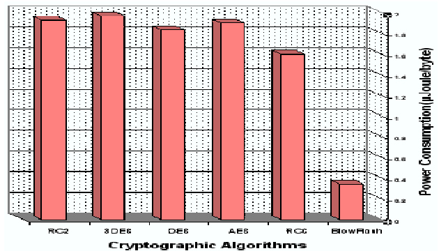
Figure 13: Power consumption for decrypting different audio files in \mu\text{Joule}/\text{Byte}
