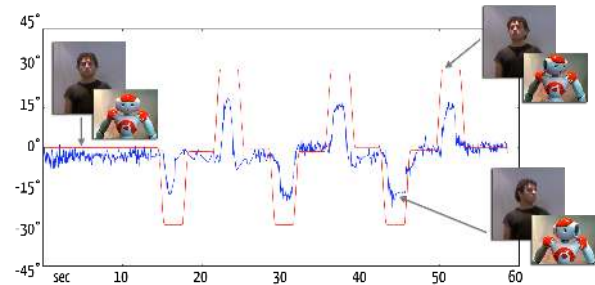
Fig. 8: The evolution over time of the robot’s head yaw, in red, overlapped to the head yaw movements of the human, in blue. This highlights several synchrony events in terms of joint attention, between the head movement of the robot and the gazing behavior of the human.
