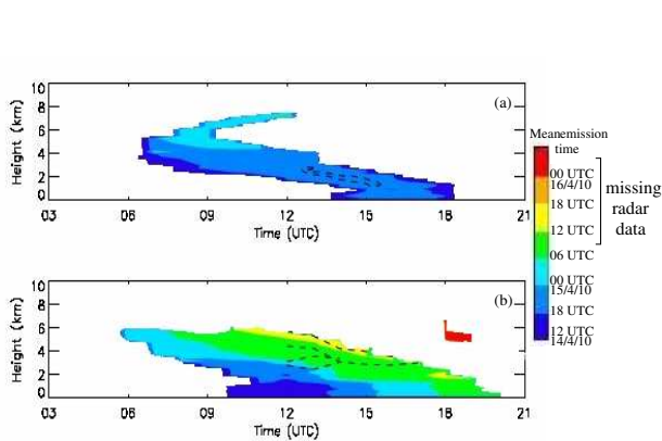
Figure 12. Time-height plots of mean emission time on 16 April 2010 at (a) Chilbolton and (b) Leipzig for the constant plume height simulation.
