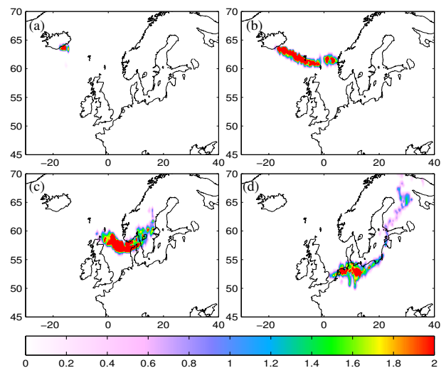
Figure 7. IASI measured volcanic ash index (K) at (a) 22 UTC on 14 April 2010, (b) 10 UTC on 15 April 2010, (c) 22 UTC on 15 April 2010 and (d) 10 UTC on 16 April 2010.
