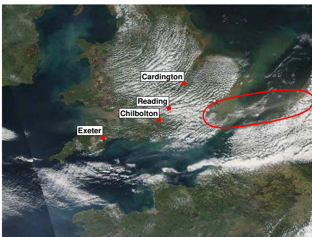
Figure 6. MODIS AQUA visible image at 13:23 UTC on 16 April showing a volcanic ash cloud (enclosed by the red contour) stretching from southern England to Belgium. The locations of the UK lidars at Cardington, Reading, Chilbolton and Exeter are overlaid.
