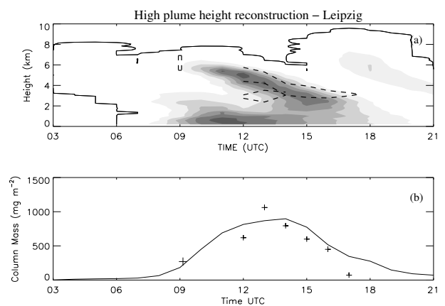
Figure 13. As figure 8 but for high plume height reconstruction simulation over Leipzig.
