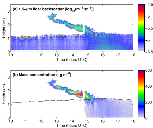
Figure 2. Time-height plots at Chilbolton ( 51.1^\circ\text{N} , 1.4^\circ\text{W} ) from 10-18 UTC on 16 April 2010. (a) lidar backscatter, and (b) mass concentration retrieved from a combination of lidar and sun photometer measurements overlaid with the boundary layer top (black line).
