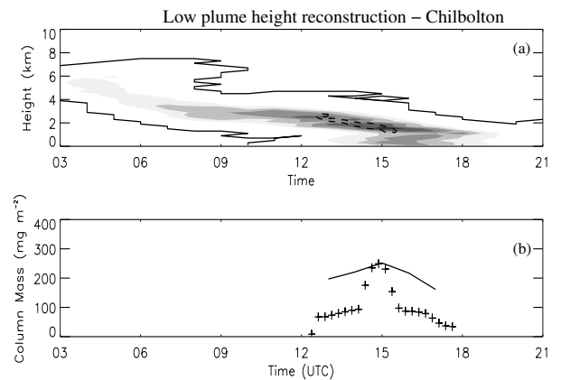
Figure 10. As figure 9 but for low plume height reconstruction simulation over Chilbolton.
