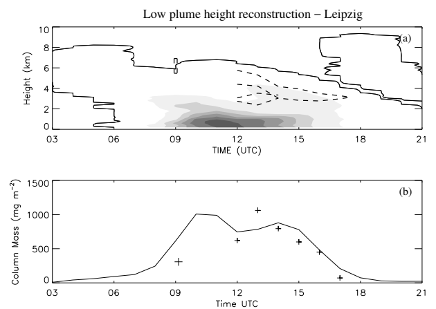
Figure 11. As figure 8 but for low plume height reconstruction simulation over Leipzig.
