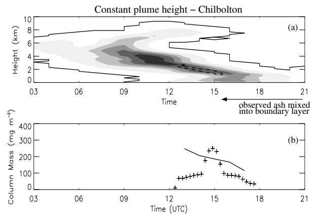
Figure 9. Constant plume height simulation on 16 April 2010. (a) Time-height plot of mass concentration over Chilbolton ( 51.1^{\circ}\text{N} , 1.4^{\circ}\text{W} ) on 16 April 2010 overlaid with the outline of the lidar ash cloud (dashed). The NAME results have been shifted by 9 hours so that the vertical structure of the NAME ash cloud and the observed ash cloud coincide. The shaded concentration contours are in arbitrary units, contours are equally spaced concentration levels and span a factor of 5. The solid black contour outlines the outermost extent of the modelled ash cloud. (b) Time-series of above boundary layer integrated mass loading over Chilbolton, from NAME (solid) and the lidar retrieval (crosses). NAME column-integrated mass loadings are only plotted for the time during which the NAME and lidar observations match.
