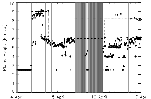
Figure 1. 5-minute time-series of plume height from the Icelandic radar (crosses), for the constant plume height simulation (solid), low plume height reconstruction (dashed) and high plume height reconstruction (dotted). The grey area represents missing radar data due to missing scans (light grey) or clouds (dark grey). The minimum plume height detectable due to mountain ranges and curvature of the Earth is 2.5 km. Where no plume is detected (but radar data isn't missing), 2.5 km has been plotted.
