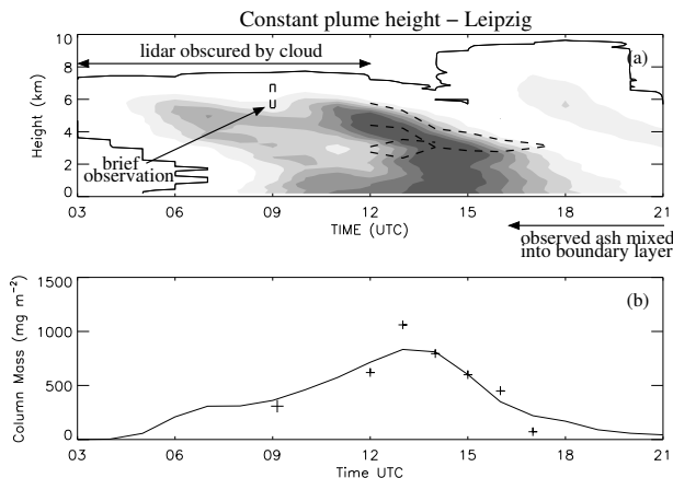
Figure 8. Constant plume height simulation on 16 April 2010. (a) Time-height plot of NAME mass concentration over Leipzig ( 51.4^{\circ}\text{N} , 12.4^{\circ}\text{E} ) on 16 April 2010 overlaid with the outline of the lidar ash cloud (dashed). The shaded concentration contours are in arbitrary units, contours are equally spaced concentration levels and span a factor of 6. The solid black contour outlines the outermost extent of the modelled ash cloud. (b) Time-series of above boundary layer integrated mass loading over Leipzig, from NAME (solid) and the lidar retrieval (crosses).
