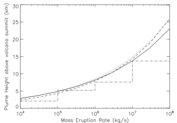
Figure 14. The variation of eruption rate with plume height used in NAME, H = 0.365M^{0.225} (solid), Mastin et al. (2009), H = 0.304M^{0.241} (dotted), Sparks et al. (1997), H = 0.220M^{0.259} (dashed) and the emission rates from the NOAA VAFTAD thresholds (dash-dot).
