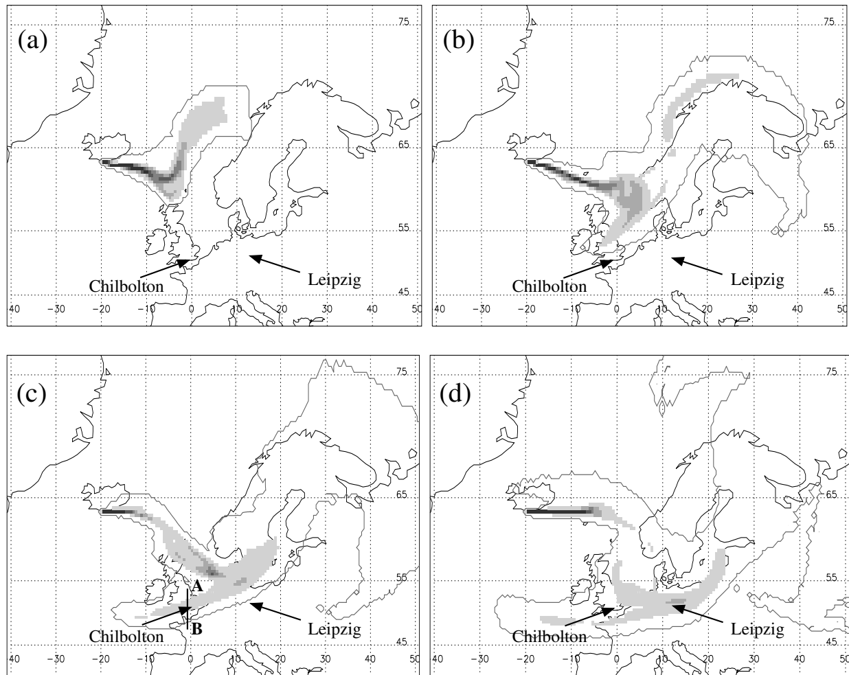
Figure 4. Column-integrated NAME mass concentration from the control simulation at (a) 00 UTC on 15 April 2010, (b) 12 UTC on 15 April 2010, (c) 00 UTC on 16 April 2010 and (d) 12 UTC on 16 April 2010. The shaded concentration contours are in arbitrary units, contours are equally spaced concentration levels and span a factor of 5 across the entire range of levels. The grey line outlines the outermost extent of the ash cloud. The black line, AB, indicates the location of the vertical cross-section in figure 5.
