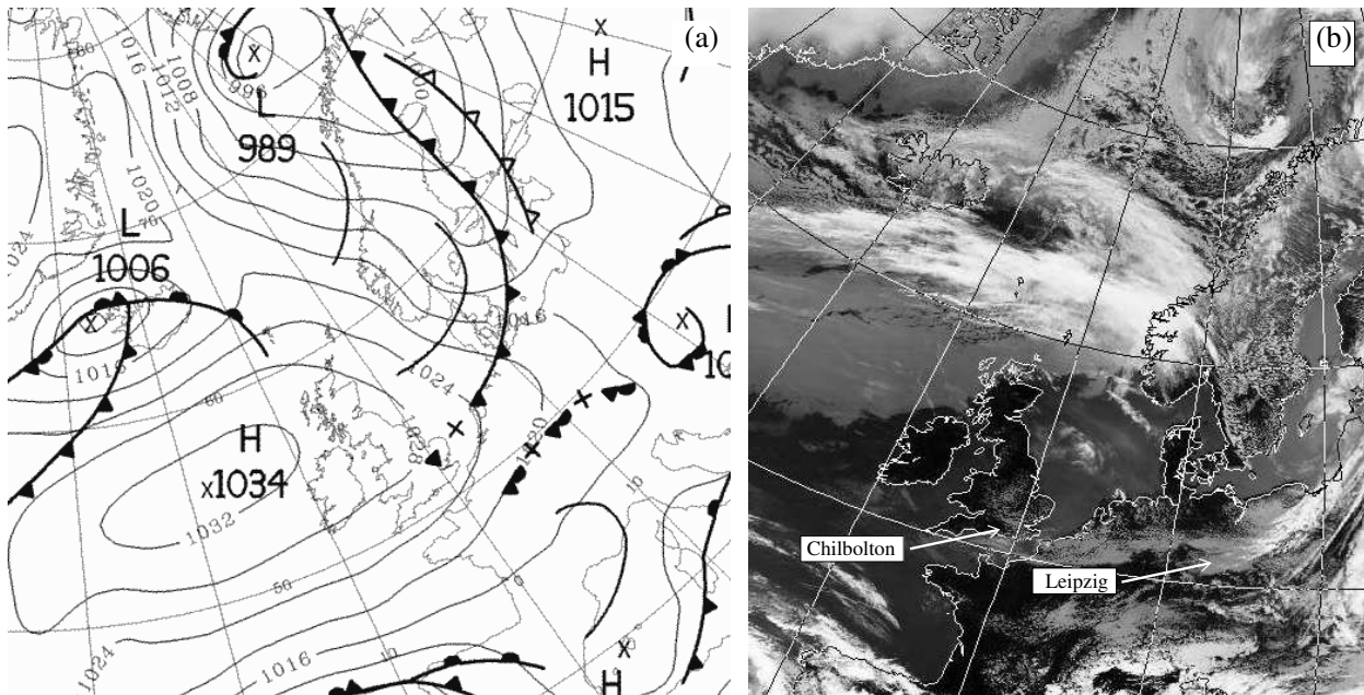
Figure 3. (a) Synoptic analysis at 00 UTC on 16 April 2010 from the UK Met Office. (b) AVHRR thermal infrared image ( 11.5 - 12.5\mu\text{m} ) at 12:55 UTC on 16 April 2010 courtesy of Dundee satellite receiving station.
