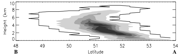
Figure 5. Vertical cross-section of mass concentration from 48^{\circ} - 54^{\circ} N at 1.4^{\circ} W (along line, AB, in figure 4(c)). The shaded concentration contours are in arbitrary units, contours are equally spaced concentration levels and span a factor of 5. The black contour outlines the outermost extent of the ash cloud.
