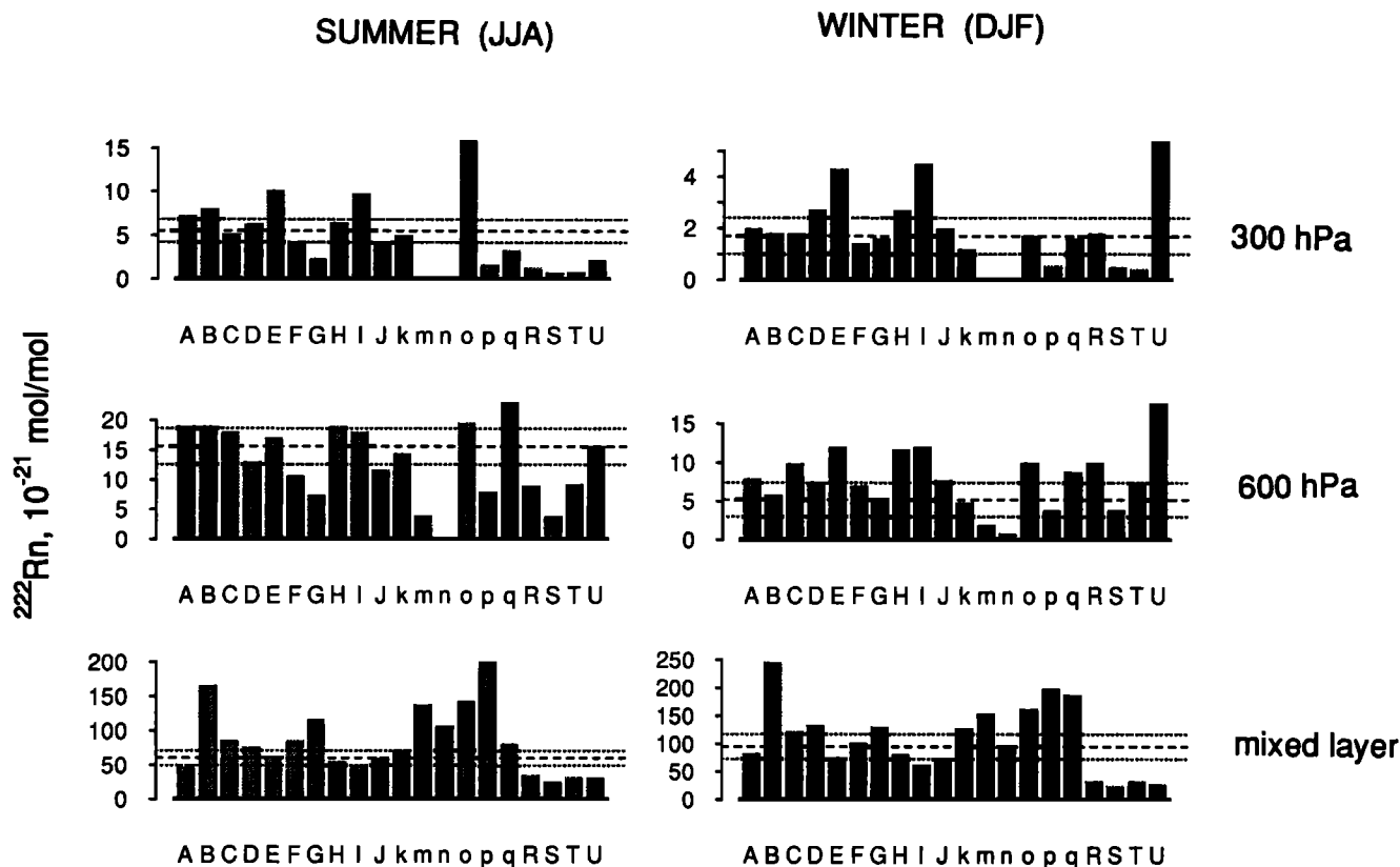
Figure 2. Mean ^{222}\text{Rn} concentrations over northern midlatitude continents at 300 m altitude (mixed layer), 600 hPa, and 300 hPa in June-August and December-February. The dashed lines are averages of aircraft observations from various locations in North America and Europe, and the dotted lines are the corresponding standard errors \sigma/\bar{n} (standard deviations on the means) [Liu et al. , 1984]. Model results are averages over the three midlatitude continental sites for which model time series were archived: Cincinnati (40°N, 84°W), Socorro (34°N, 107°W), and Kirov (58°N, 49°E). The models are identified by the letter code of Table 1.
