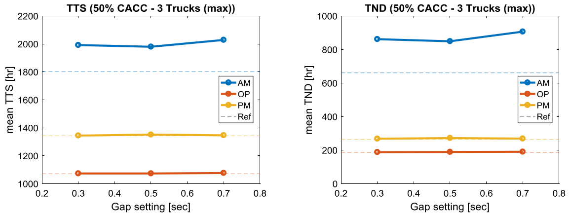
Fig. 7. A–b. TTS and TND for three-truck platoons (dashed lines show reference scenario without platooning).
