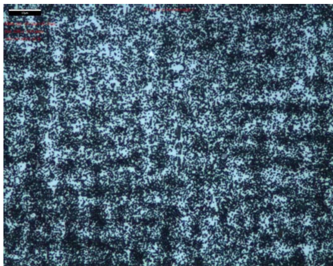
Figure 4: solar cell with 2D texturing without nitride antireflection.
