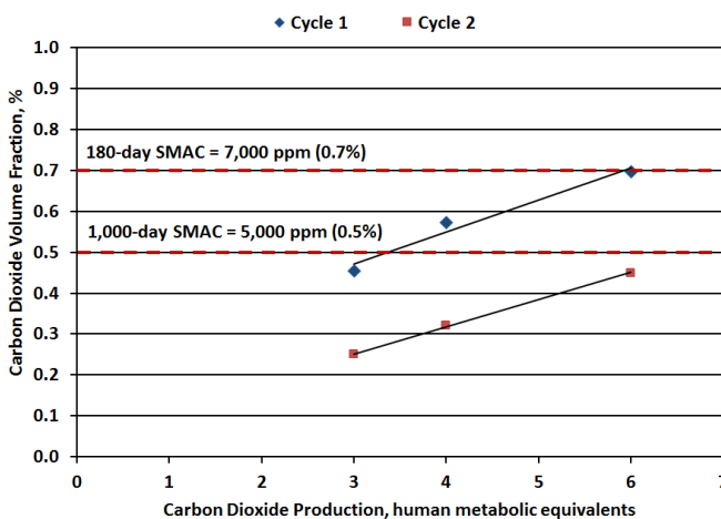
Figure 9. Comparison of Average \text{CO}_2 partial pressure plateau concentrations during the ARREM Cycle 1 and Cycle 2 tests. Single person \text{CO}_2 production basis is 0.042
