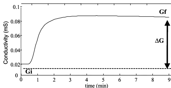
Fig. 5. Response of sensor TGS-800 to fruit aroma ( T = 20\text{ }^{\circ}\text{C} ; RH 75%). The curve represents the conductance transient (mS) of a single sensor under a step change in the concentration of fruit aroma. The graphical meaning of three static parameters ( G_i , G_f , and \Delta G ) is illustrated.
