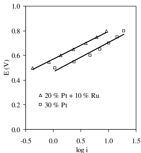
Figure 3. Polarization curves for the electro-oxidation of 0.2 M CH 3 OH in 0.5 M H 2 SO 4 on 30 % Pt and 20 % Pt + 10 % Ru catalysts. The current-potential data were obtained from the analysis of the rising portion of forward anodic peak of the electro-oxidation of 0.2 M CH 3 OH in 0.5 M H 2 SO 4 at 50 mV s -1 scan rate.
