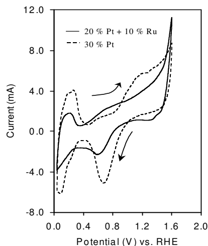
Figure 1. Comparison of the hydrogen adsorption region of the cyclic voltammogram of 30 % Pt and 20 % Pt + 10 % Ru catalysts at 50 \text{ mV s}^{-1} scan rate in 0.5 \text{ M H}_2\text{SO}_4 .
