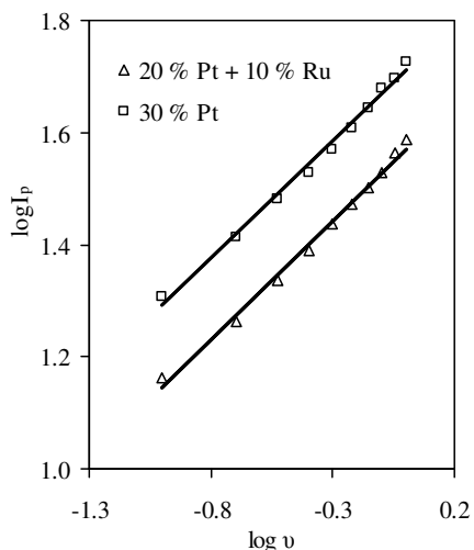
Figure 4. Plots of logarithm of peak current “ \log I_p ” vs. the logarithm of scan rate “ \log v ” for the electro-oxidation of methanol in 0.5 M H_2SO_4 on 30 % Pt and 20 % Pt + 10 % Ru catalysts.
