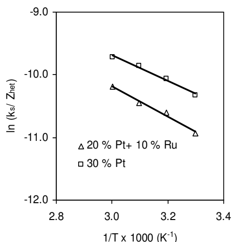
Figure 6. Plots of \ln k_s / Z_{\text{het}} vs. 1/T for evaluation of thermodynamic parameters of the electro-oxidation of methanol in 0.5 M \text{H}_2\text{SO}_4 on 30 % Pt and 20 % Pt + 10 % Ru catalysts.
