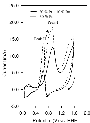
Figure 2. Comparison of the cyclic voltammogram of 30 % Pt and 20 % Pt + 10 % Ru catalysts in 0.2 M CH 3 OH + 0.5M H 2 SO 4 at 50 mV s -1 scan rate.
