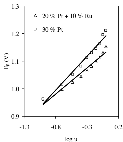
Figure 5. Plots of peak potential “ E_p ” vs. the logarithm of scan rate “ \log v ” for the electro-oxidation of methanol in 0.5 M H_2SO_4 on 30 % Pt and 20 % Pt + 10 % Ru catalysts.
