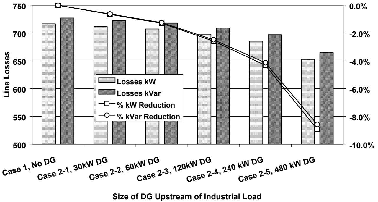
Fig. A.6. System loss reduction provided by DER up steam of load point
